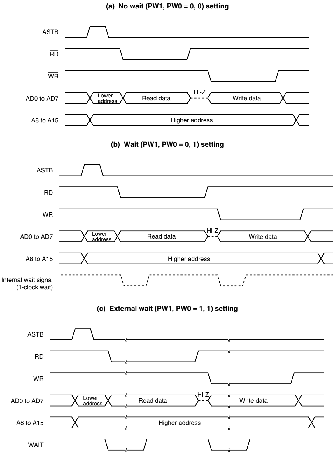
Figure 5-8. External Memory Read Modify Write Timing
