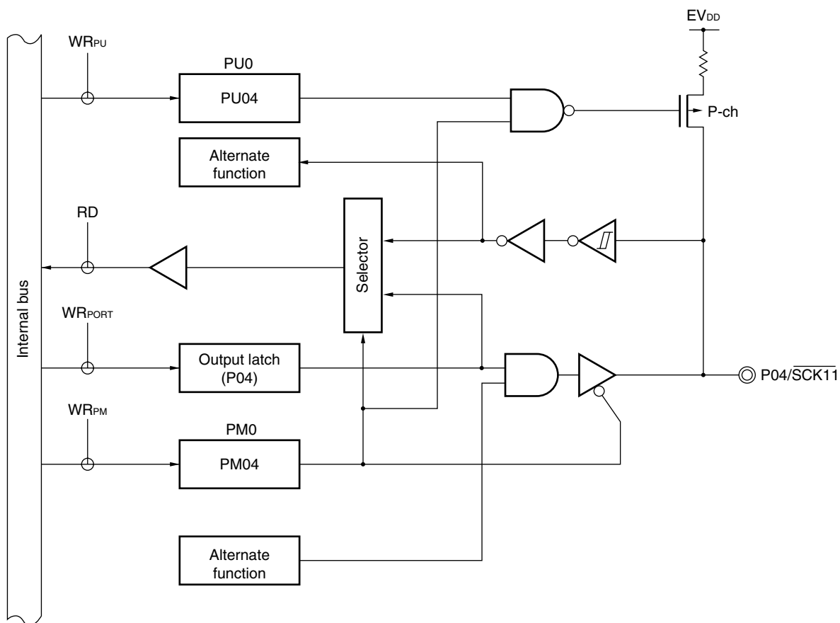
Figure 4-5. Block Diagram of P04
