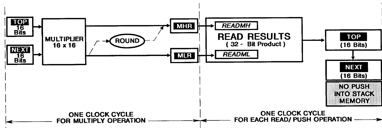
FIGURE 16. MULTIPLIER OPERATION
