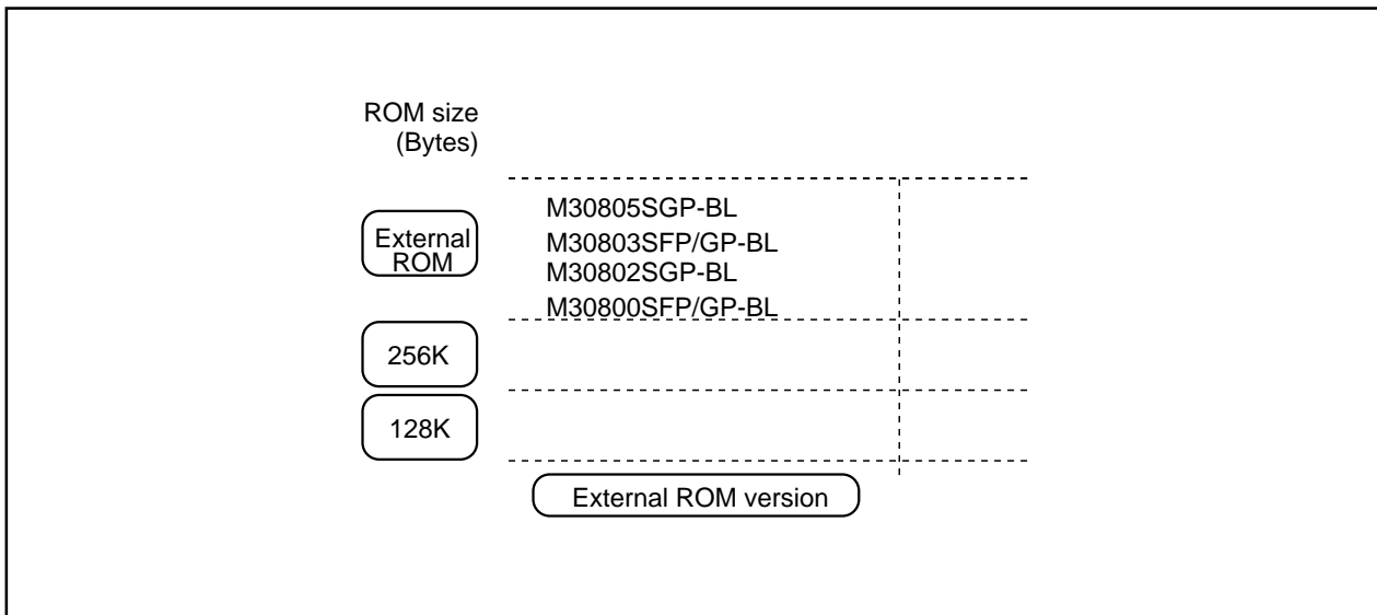
Figure 33.1 ROM Expansion
