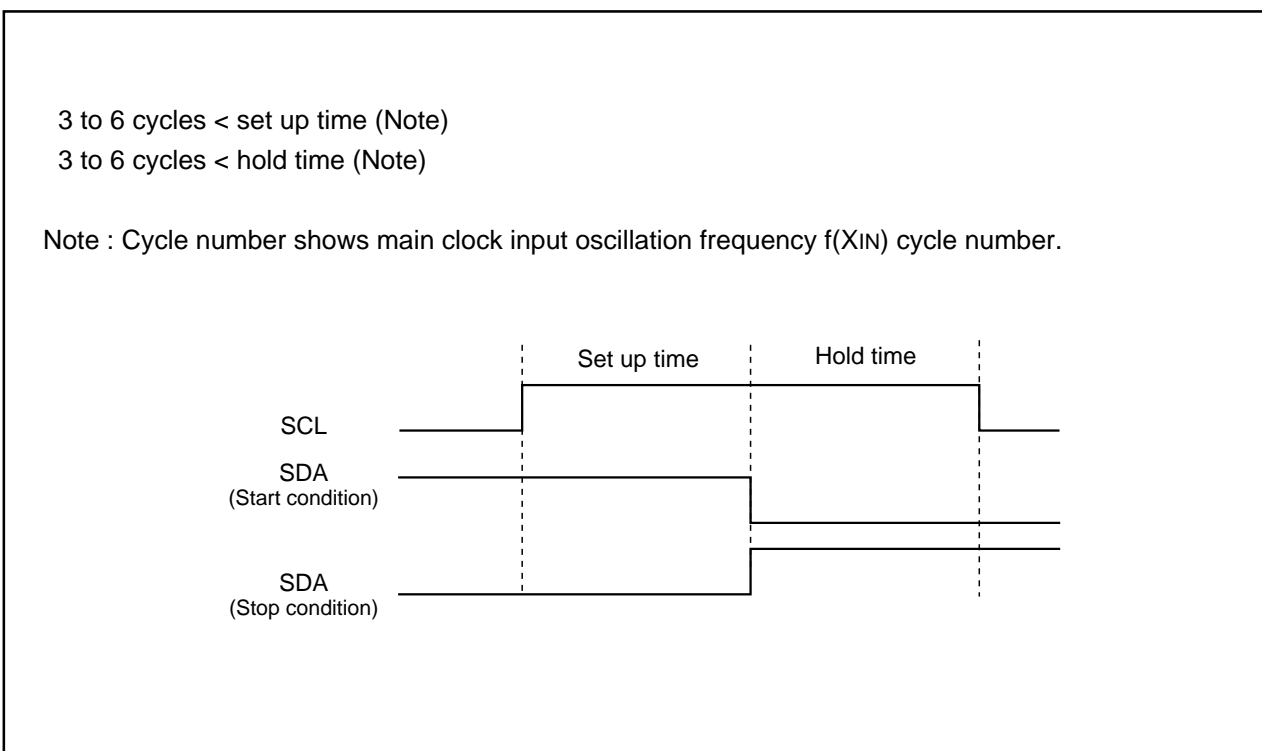
Figure 20.4 Start/stop condition detect timing characteristics
