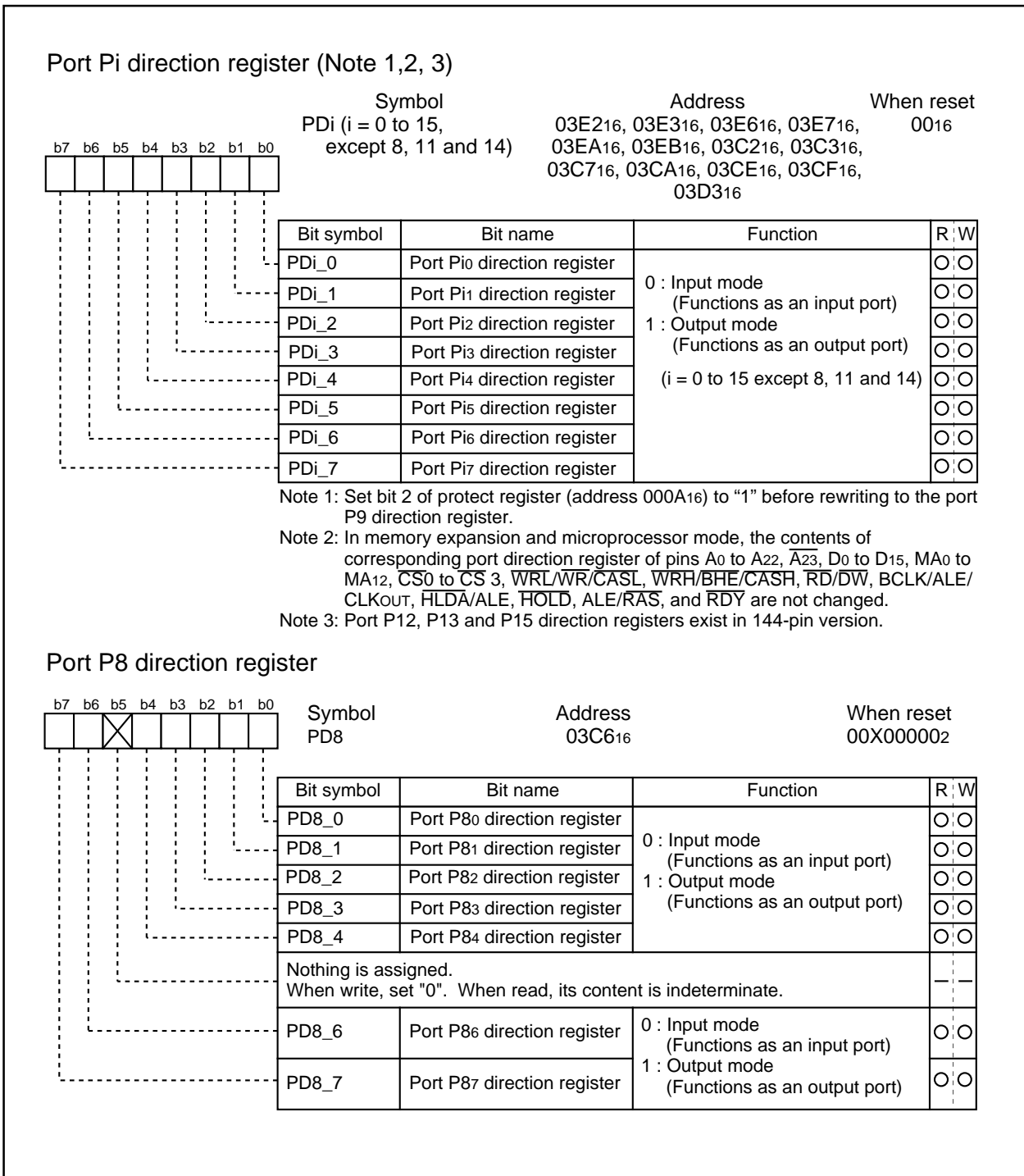
Figure 26.4 Direction register (1)
