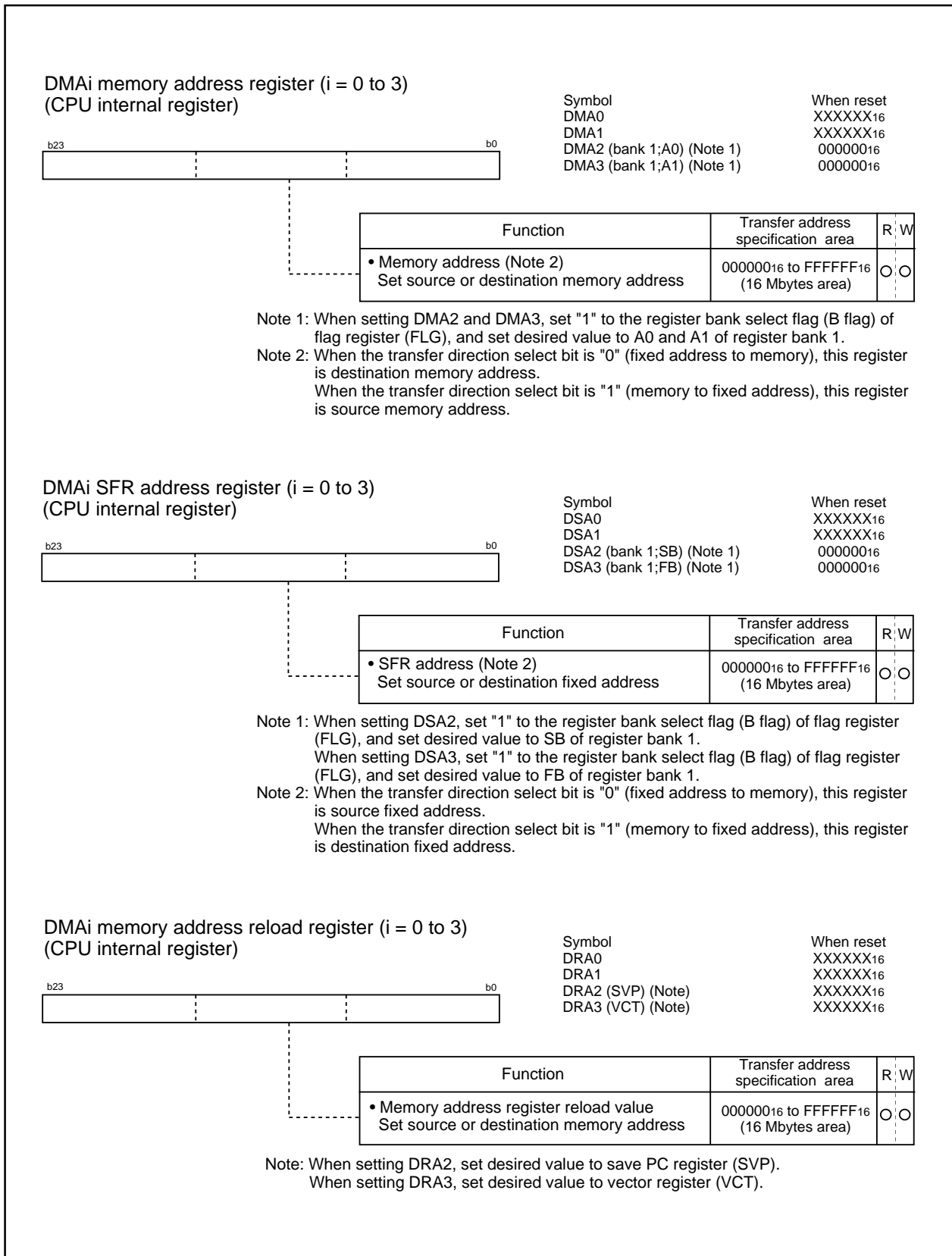
Figure 11.5 DMAC register (4)
