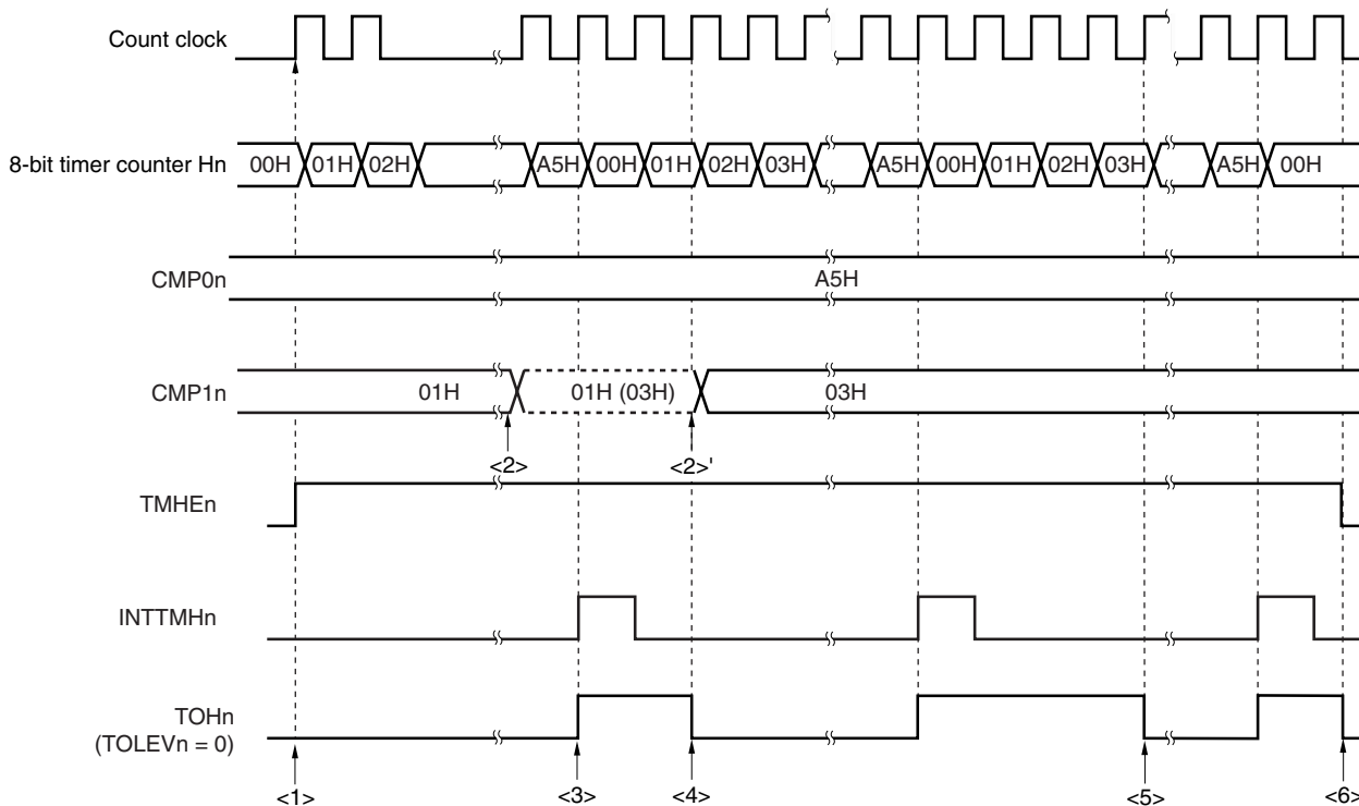
(e) Operation by changing CMP1n (CMP1n = 01H → 03H, CMP0n = A5H)
