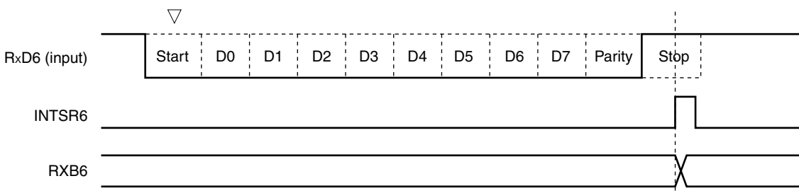
Figure 13-19. Reception Completion Interrupt Request Timing
