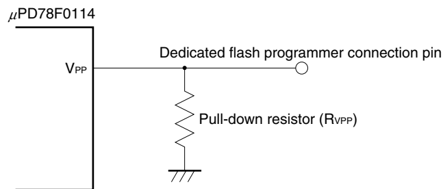
Figure 23-13. Example of Connection of V_{PP} Pin
