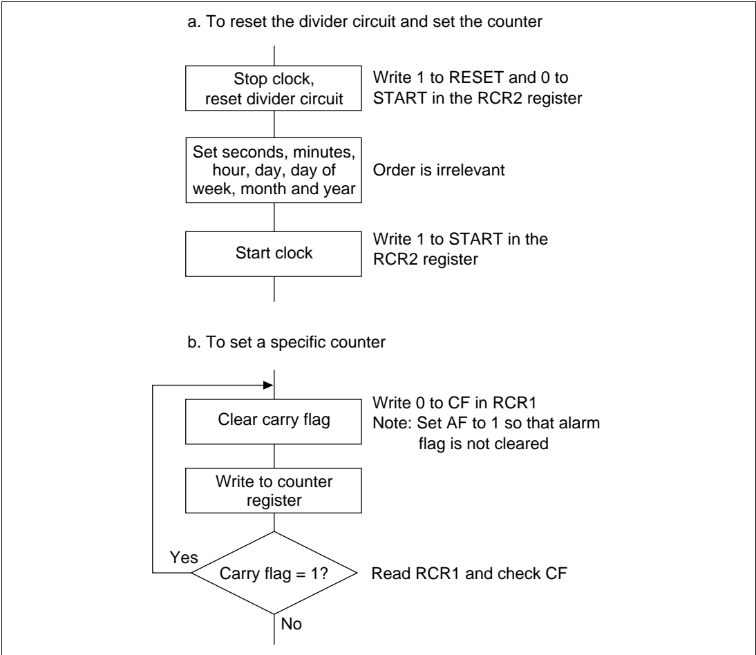
Figure 14.2 Setting the Time
