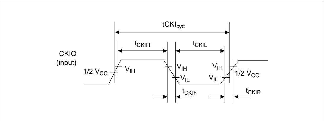
Figure 24.2 CKIO Clock Input Timing
