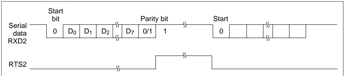
Figure 17.12 Example of Operation Using Modem Control (RTS2)
