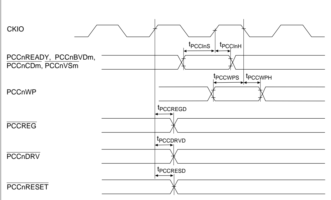
Figure 24.51 PCC Input/Output Timing
