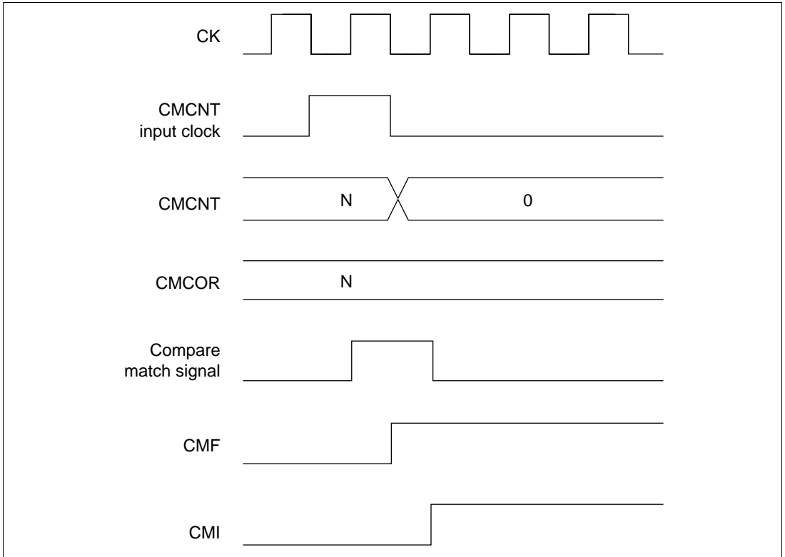
Figure 12.21 Timing of CMF Setting
