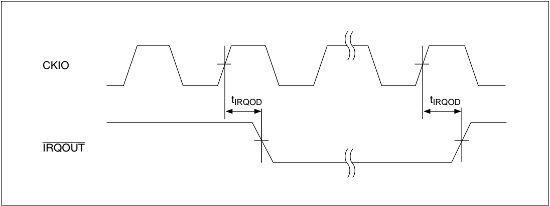
Figure 24.14 \overline{\text{IRQOUT}} Timing
