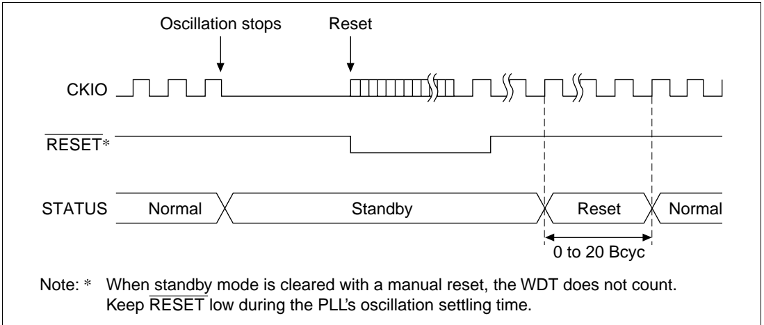
Figure 8.10 Sleep to Power-On Reset STATUS Output
