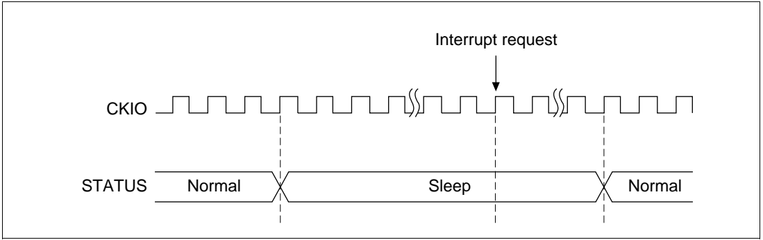
Figure 8.9 Sleep to Interrupt STATUS Output
