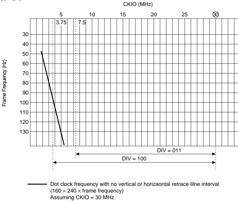
Figure 21.12 Relationship between CKIO and Frame Frequency (cont)
