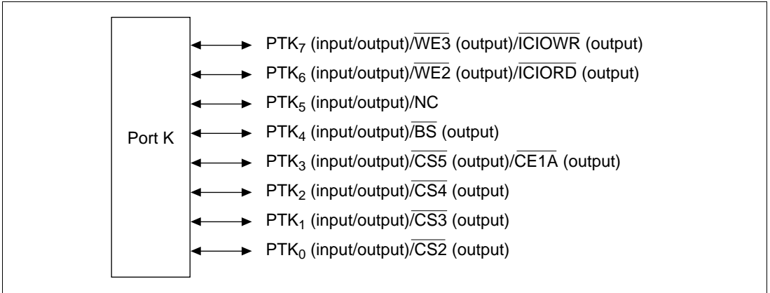
Figure 20.10 Port K
