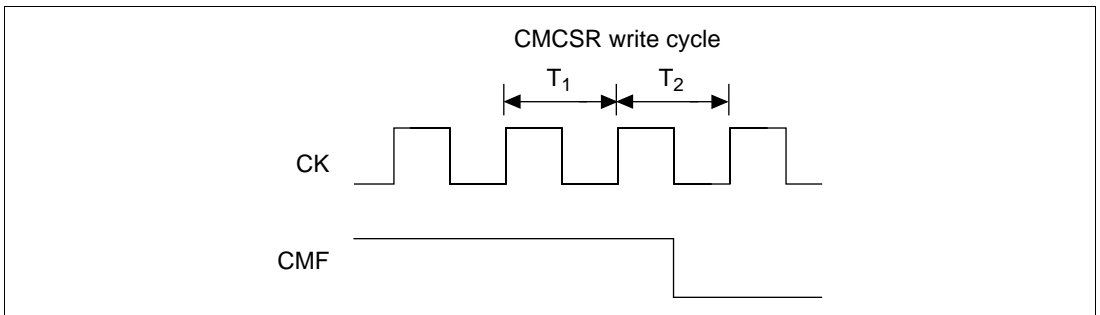
Figure 12.22 Timing of CMF Clearing by the CPU
