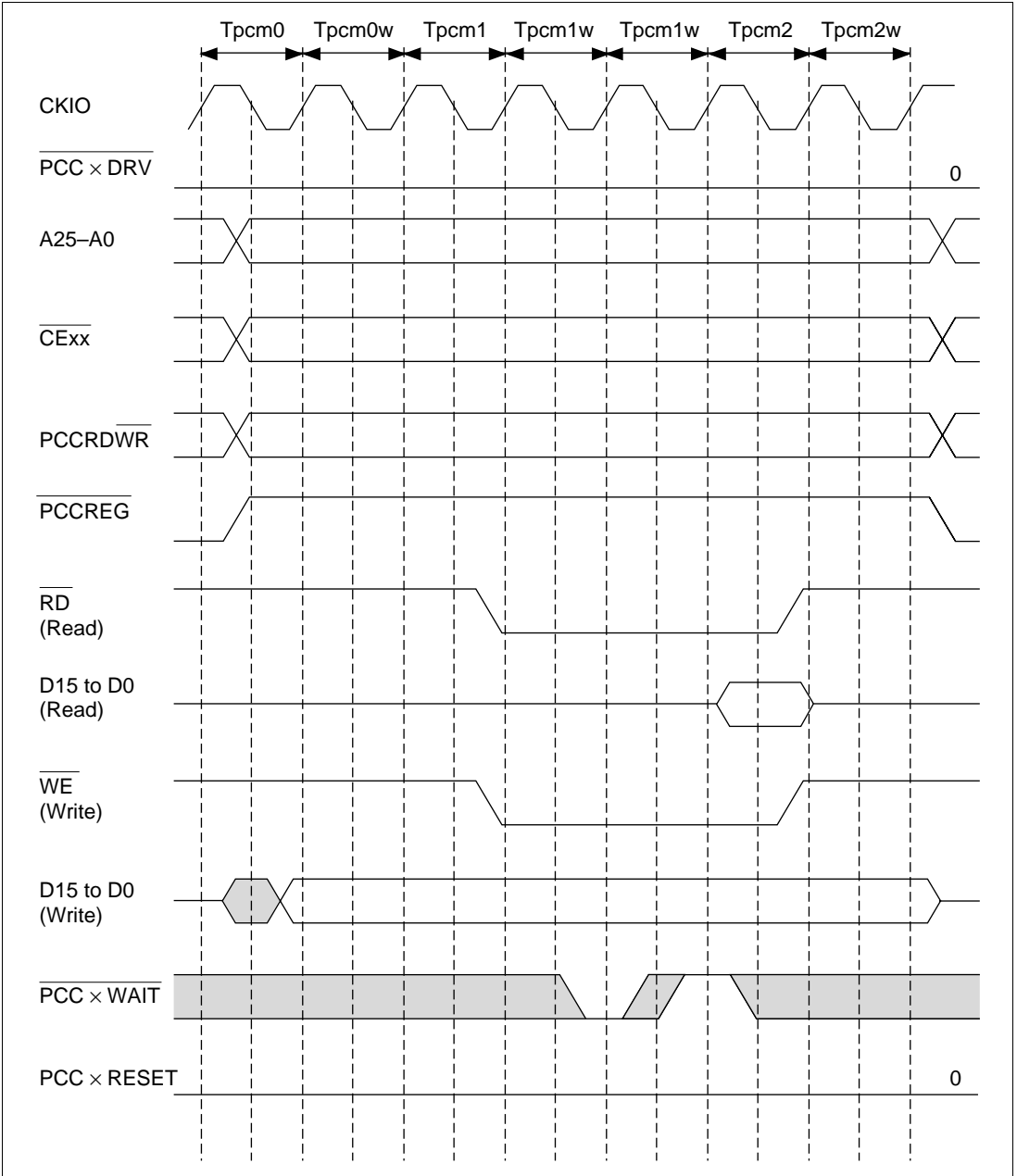
Figure 11.7 PCMCIA Memory Card Interface Wait Timing
