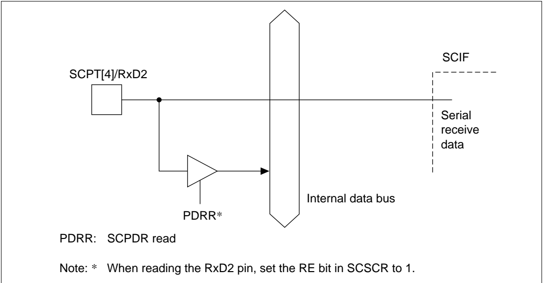
Figure 17.4 SCPT[4]/RxD2 Pin
