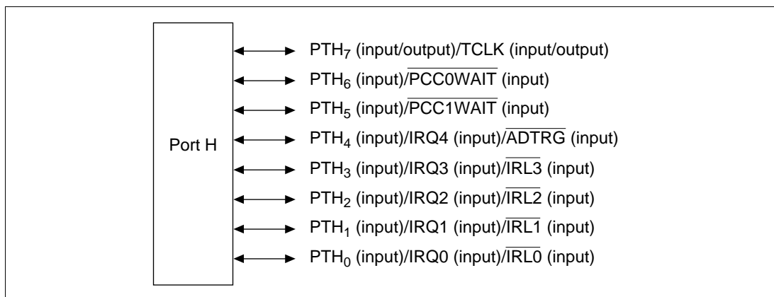
Figure 20.8 Port H
