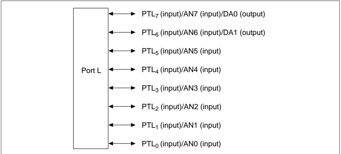
Figure 20.11 Port L
