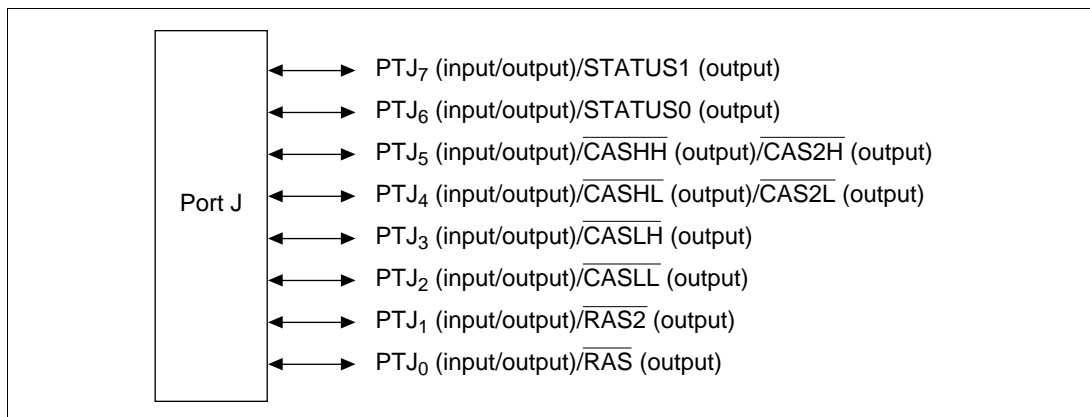
Figure 20.9 Port J
