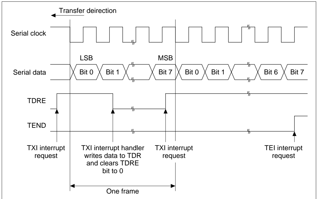
Figure 15.20 Example of SCI Transmit Operation
