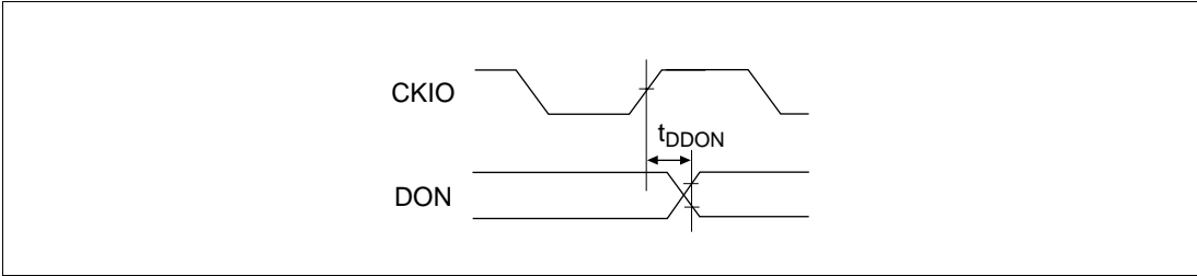
Figure 24.53 DON Output Timing
