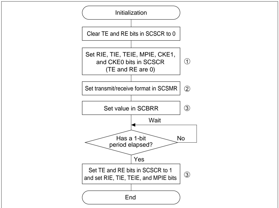
Figure 15.18 Sample Flowchart for SCI Initialization
