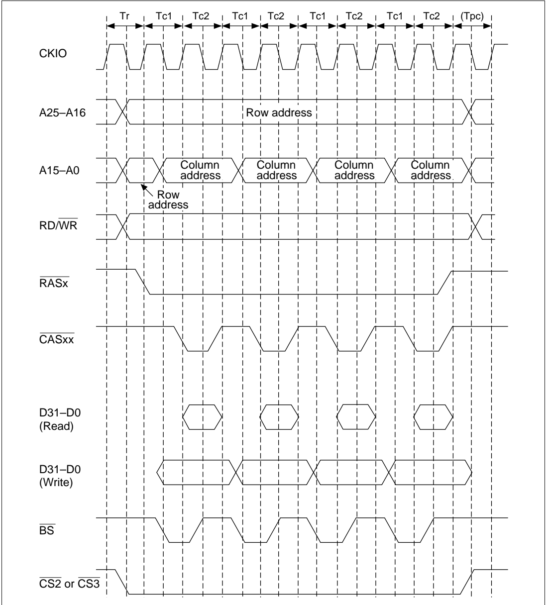
Figure 10.17 DRAM Burst Access Timing
