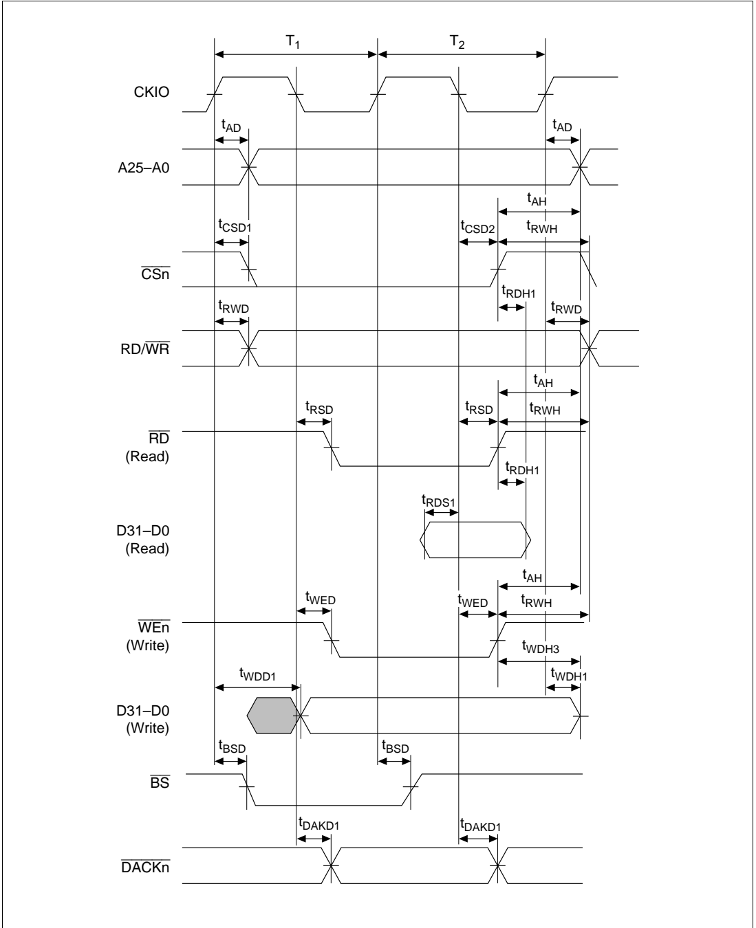
Figure 24.17 Basic Bus Cycle (No Wait)
