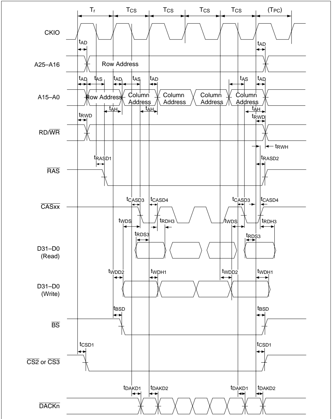
Figure 24.32 DRAM Short-Pitch Burst Access Timing
