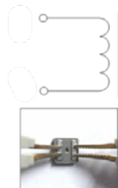
Figure 1. DCR test
