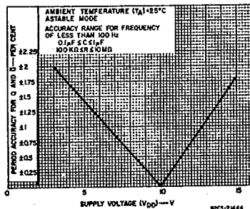
Fig. 13 - Typical Q-and-Q-bar-period accuracy vs supply voltage (very low frequency).
