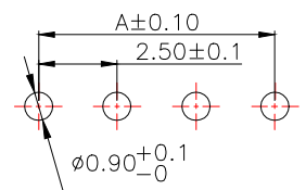
SUGGESTED PCB LAYOUT (COMPONENT SIDE)
