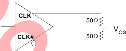
Figure 9. Output Offset Voltage
