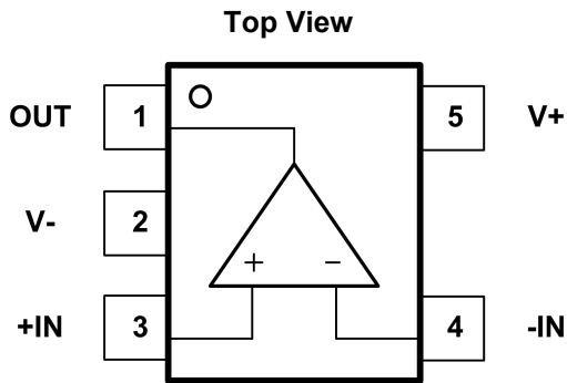
Fig. 5-1. GT8551: S5(SOT23-5) Package GT8551: C5(SC70-5) Package
