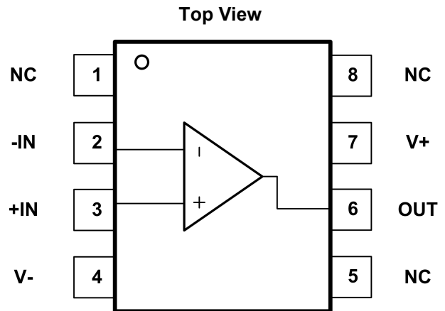
Fig.5-2. GT8551: P8(SOP8/ SOIC-8) Package GT8551: M8(MSOP8) Package
