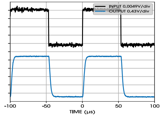
Figure 17. Large Signal Step Response (Gain = 100)
