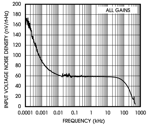
Figure 21. Input Voltage Noise Density vs. Frequency
