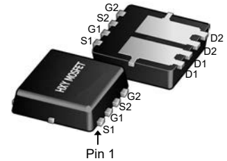
DFN3X3-8L
