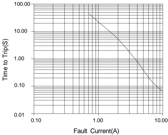
SMD0805-035/30N Fault current chart
