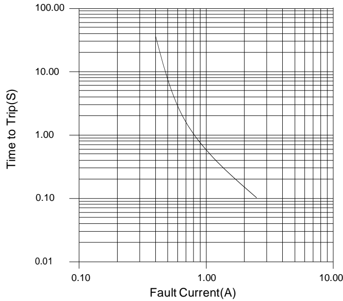
SMD0603-020/16N Fault current chart
