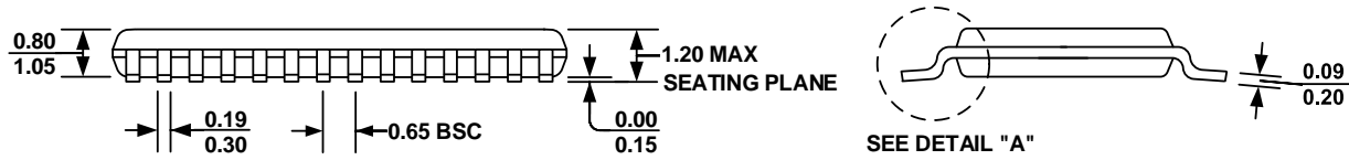
FRONT VIEW
