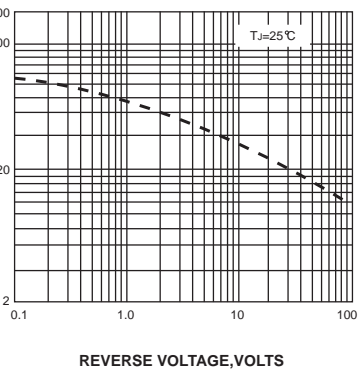
FIG. 5-TYPICAL JUNCTION CAPACITANCE
