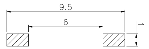
PCB. 焊接图 PCB. WELDING DRAWING
