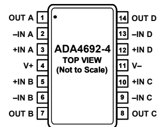
Figure 8. TSSOP-14 (RU-14)
