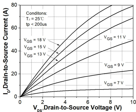
Figure 2. Output characteristics T_J = 25\text{ }^\circ\text{C}
