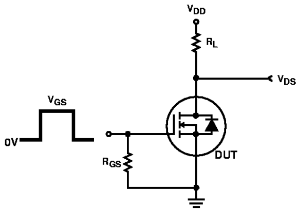
FIGURE 12. RESISTIVE SWITCHING TEST CIRCUIT
