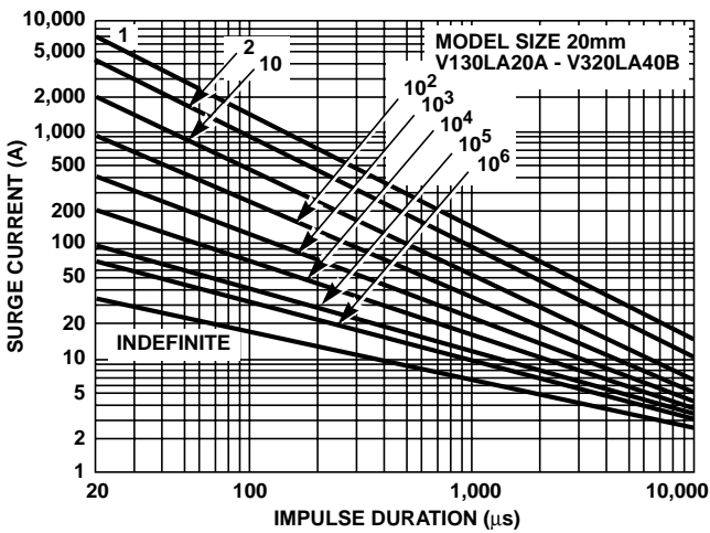
FIGURE 18. SURGE CURRENT RATING CURVES FOR V130LA20A - V320LA40B
