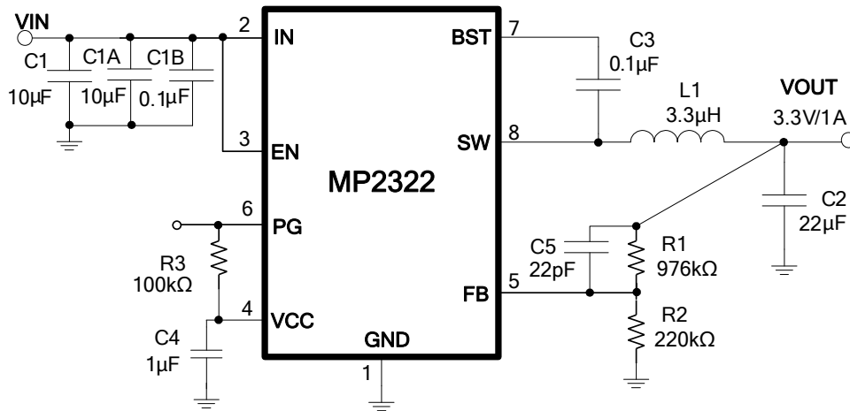
Figure 8: V IN = 12V, V OUT = 3.3V, I OUT = 1A
