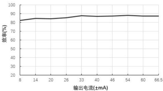
效率Vs输出电流(Vin=5V)@E0515S-2WR3
