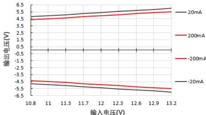
输出电压Vs输入电压@E1205S-2WR3
