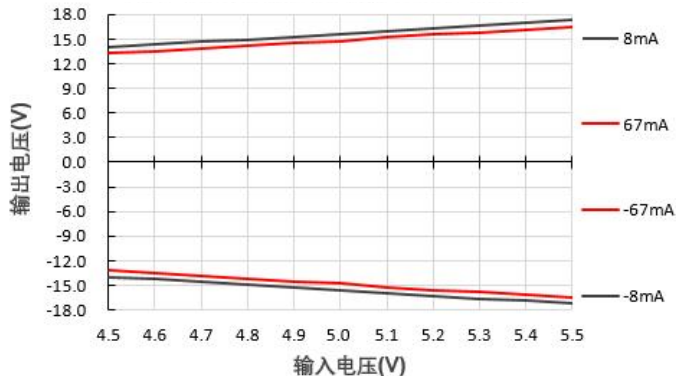
输出电压Vs输入电压@E0515S-2WR3
