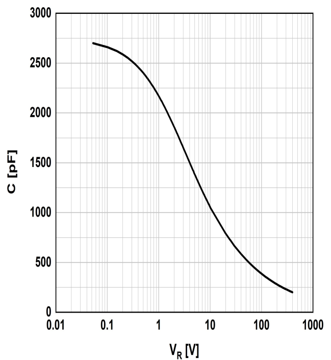
Figure.8 Capacitance vs. reverse voltage
