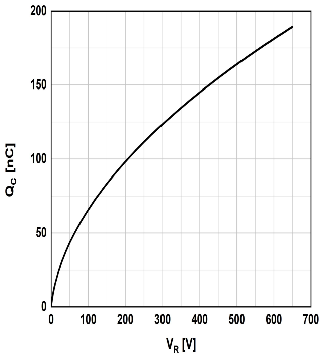
Figure.5 Capacitance charge vs. reverse voltage
