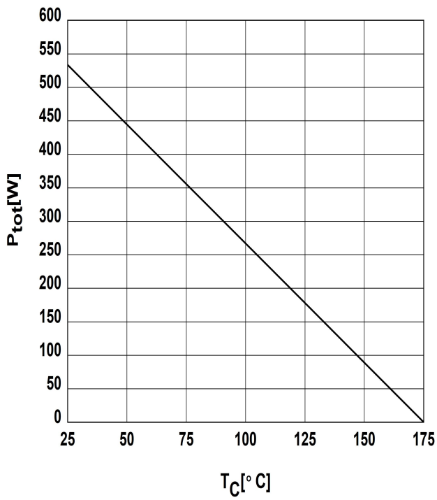
Figure.1 Power dissipation
