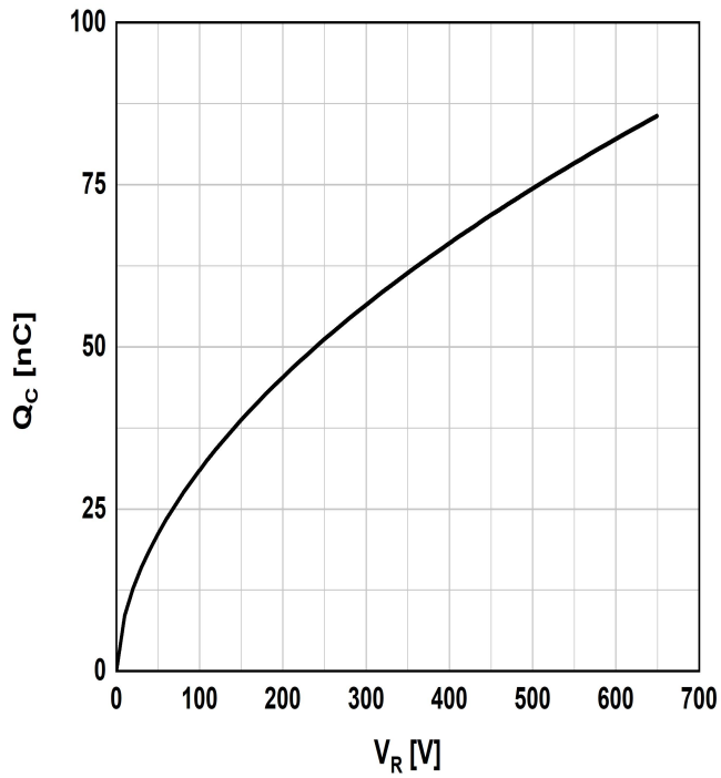
Figure.5 Capacitance charge vs. reverse voltage
