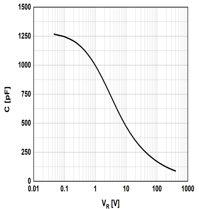
Figure.8 Capacitance vs. reverse voltage
