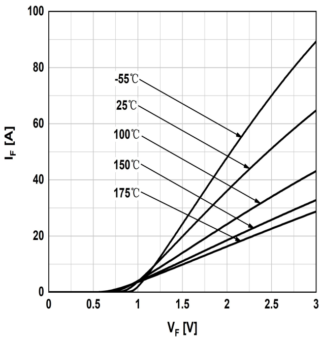
Figure.3 Typical forward characteristics
