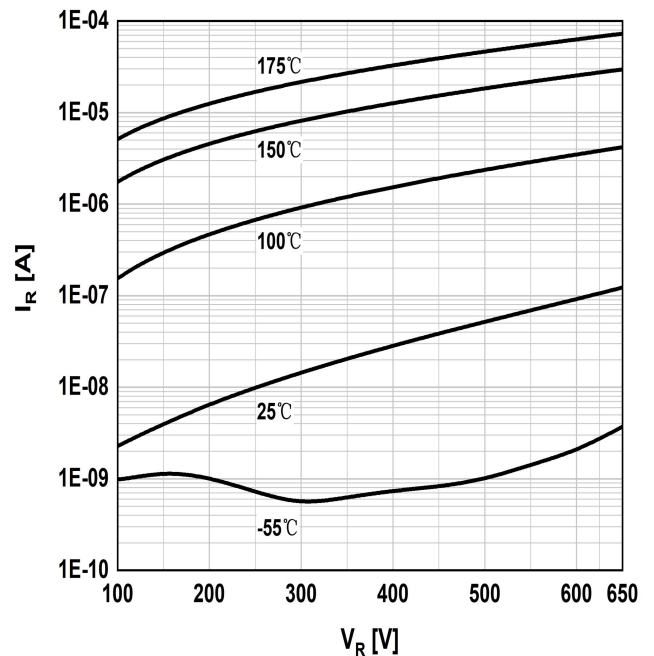
Figure.4 Reverse current vs. reverse voltage
