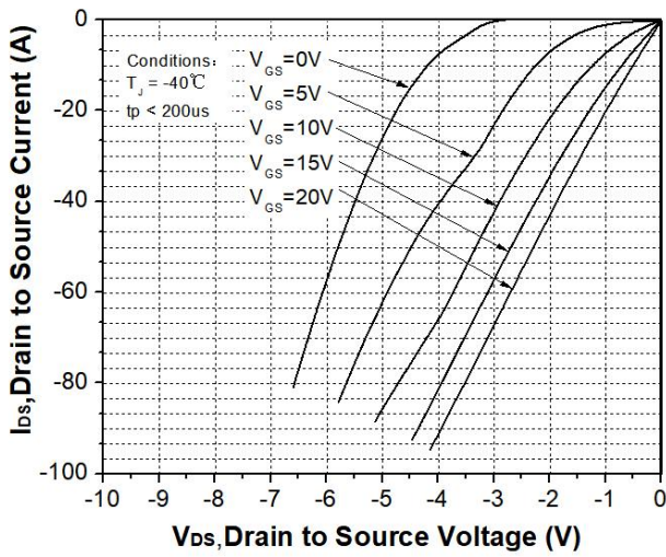
Figure 13. 3rd quadrant characteristic at T_j = -40^\circ\text{C}
