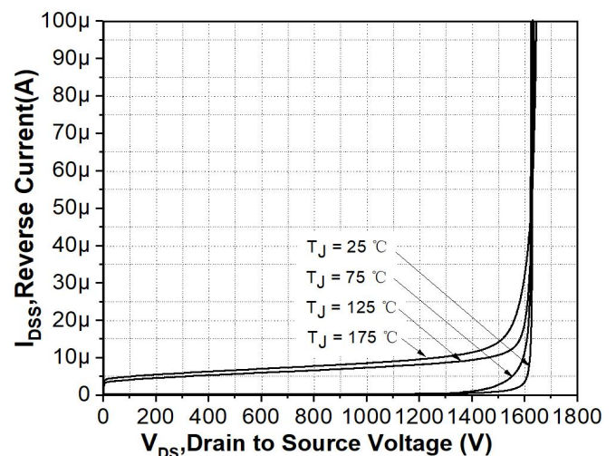
Figure 28. Reverse characteristics vs. T_J
