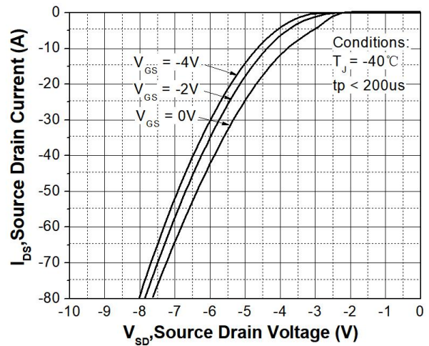
Figure 8. Body diode characteristic at T_J = -40^\circ\text{C}
