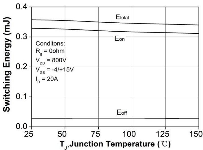
Figure 25. Clamped inductive switching energy vs. temperature
