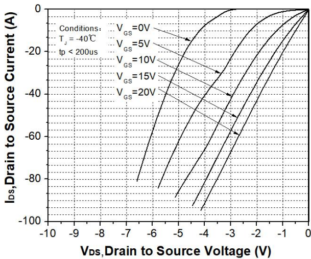
Figure 13. 3rd quadrant characteristic at T_j = -40^\circ\text{C}
