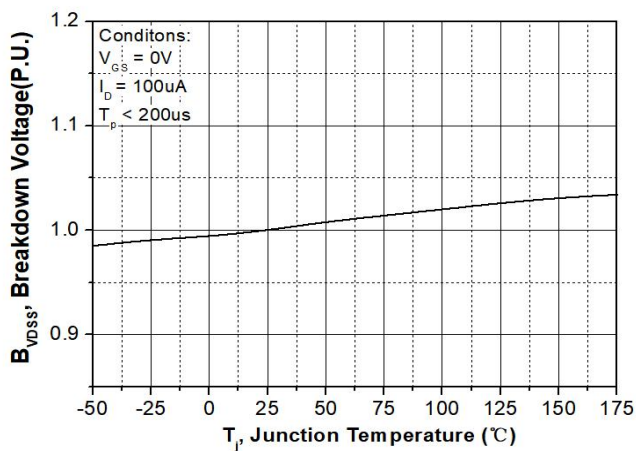
Figure 27. Reverse characteristics vs. T_J
