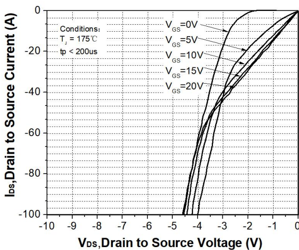
Figure 15. 3rd quadrant characteristic at T_j = 175^\circ\text{C}
