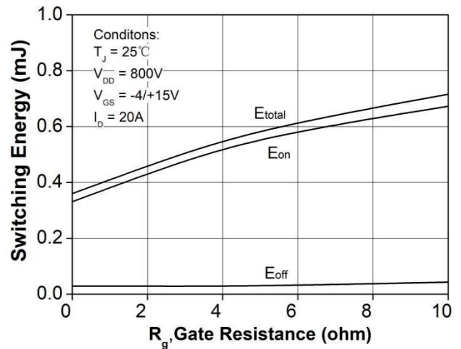
Figure 24. Clamped inductive switching energy vs. R_G(\text{ext})
