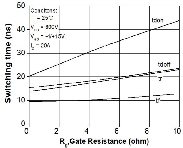
Figure 26. Switching times vs. R_G(\text{ext})
