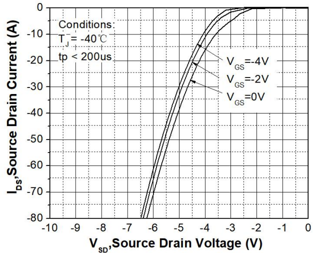
Figure 8. Body diode characteristic at T_J = -40\text{ }^\circ\text{C}
