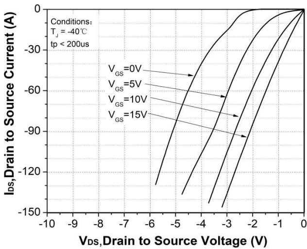
Figure 13. 3rd quadrant characteristic at T_J = -40^\circ\text{C}
