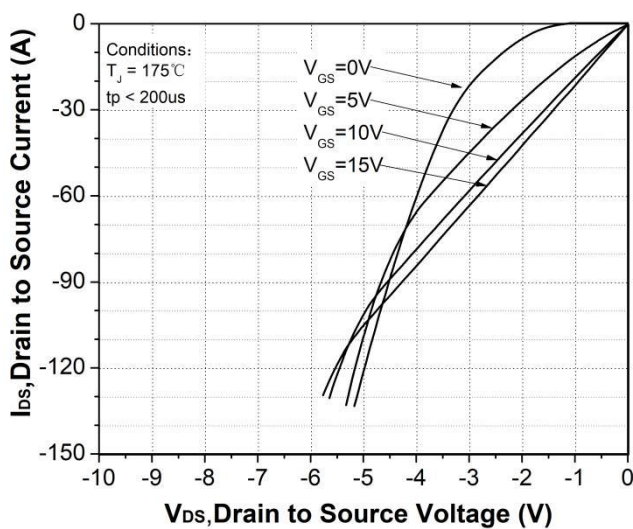
Figure 15. 3rd quadrant characteristic at T_J = 175^\circ\text{C}
