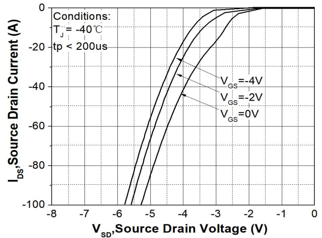
Figure 8. Body diode characteristic at T_J = -40\text{ }^\circ\text{C}
