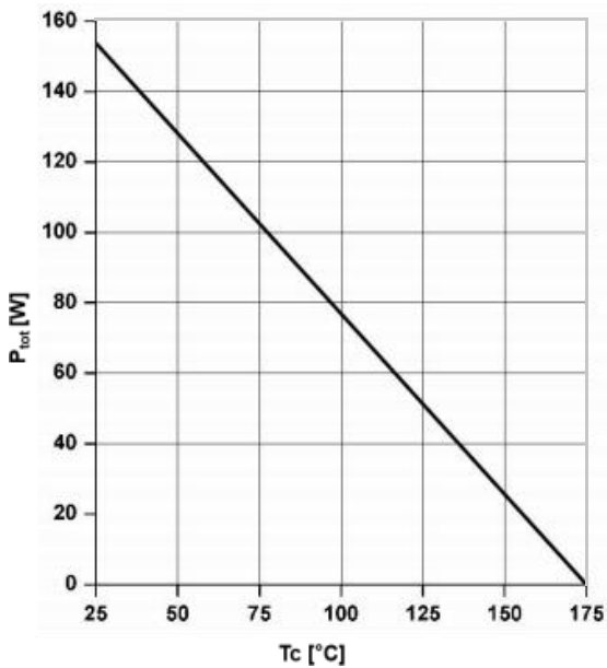
Figure.7 Power dissipation
