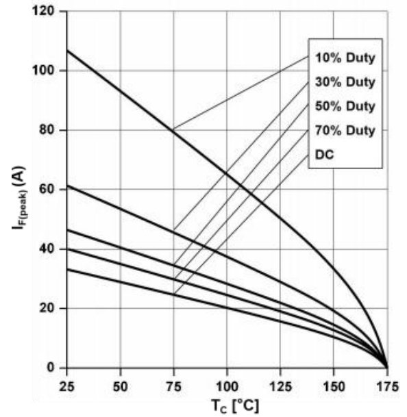
Figure.6 Diode forward current
