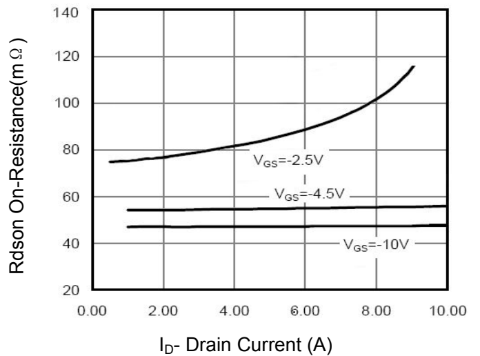
Figure 6 Drain-Source On-Resistance
