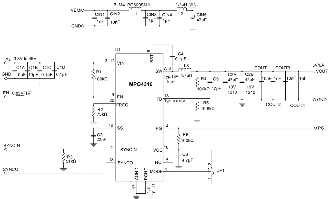
Figure 14: V OUT = 5V, f sw = 410kHz with EMI Filters
