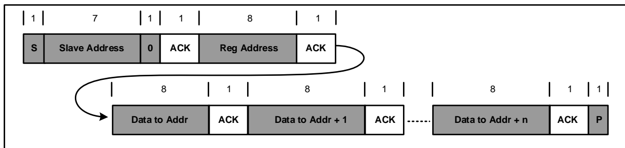
Figure 14: Multi-Write
