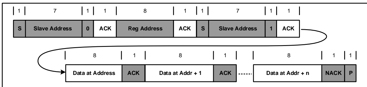
Figure 15: Multi-Read
