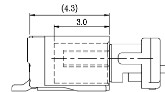
MATED CONDITION
