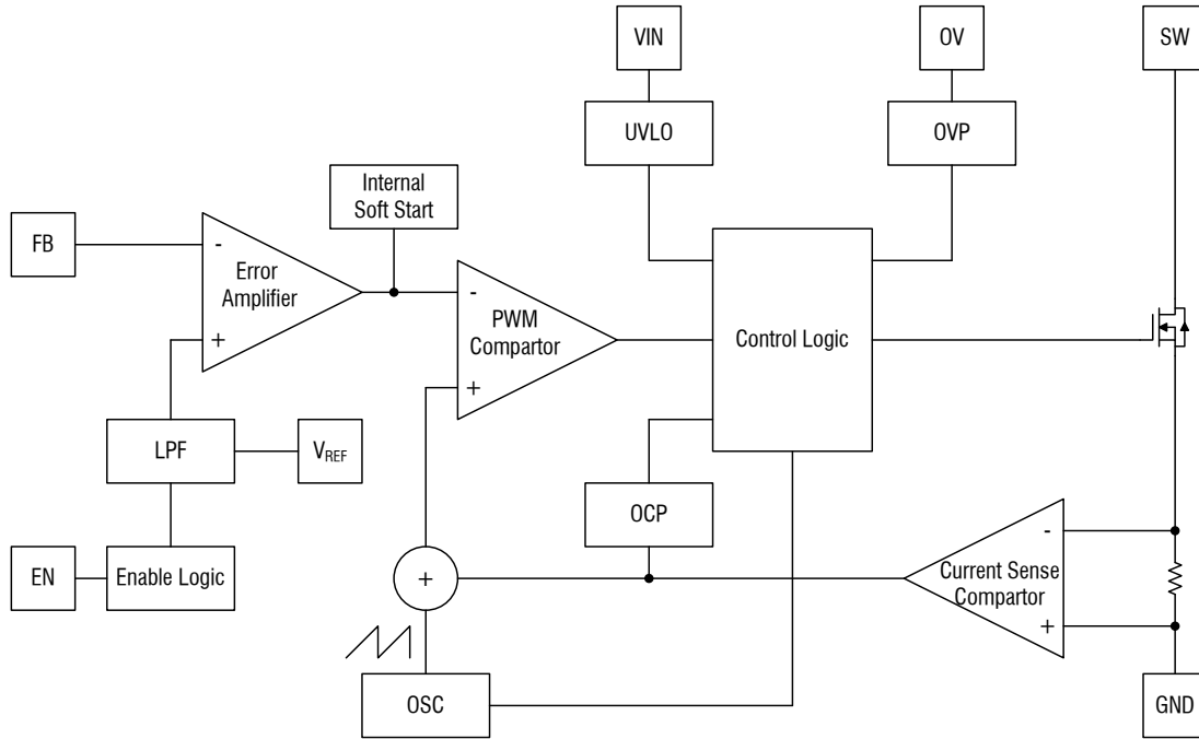
Figure 2. TCS5530 Block Diagram
