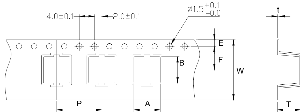
Fig. 6 Carrier tape
