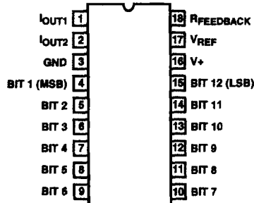
AD7521, AD7531 (PDIP) TOP VIEW
