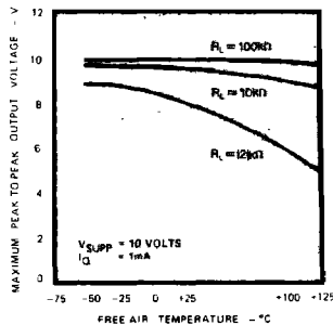
MAXIMUM PEAK-TO-PEAK VOLTAGE AS A FUNCTION OF FREE-AIR TEMPERATURE
