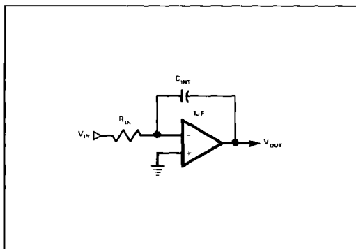
Figure 10. Long Time Constant Integrator — With R_{IN} = 10^{11} ohm, the time constant of this integrator is 100,000 seconds. Since the input voltage is converted to a current by R_{IN} , the input voltage can far exceed the power supply voltage.
