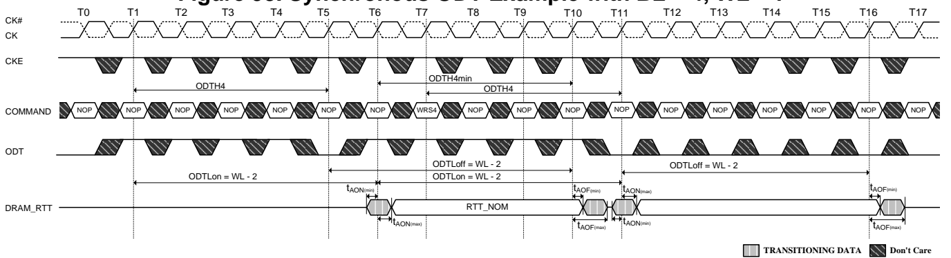
Figure 93. Synchronous ODT Example with BL = 4, WL = 7
