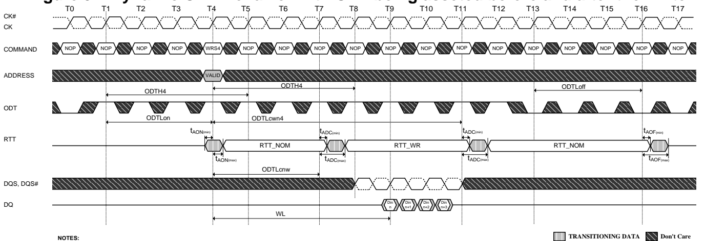
Figure 94. Dynamic ODT Behavior with ODT being asserted before and after the Write
