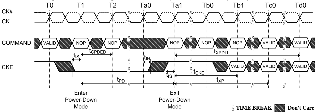
Figure 87. Precharge Power-Down (Slow Exit Mode) Entry and Exit
