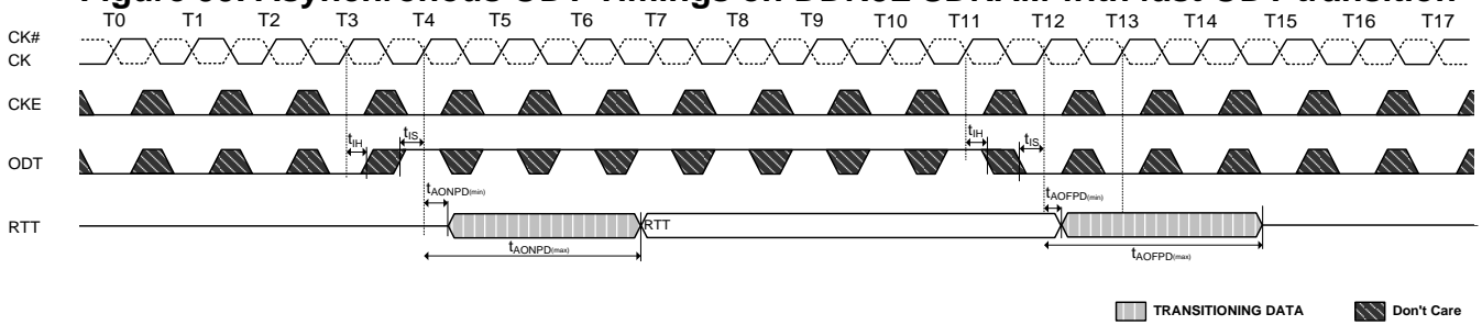
Figure 99. Asynchronous ODT Timings on DDR3L SDRAM with fast ODT transition
