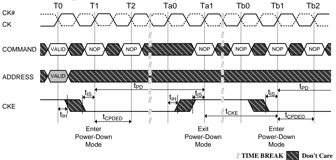
Figure 104. Power-Down Entry, Exit Clarifications-Case 1
