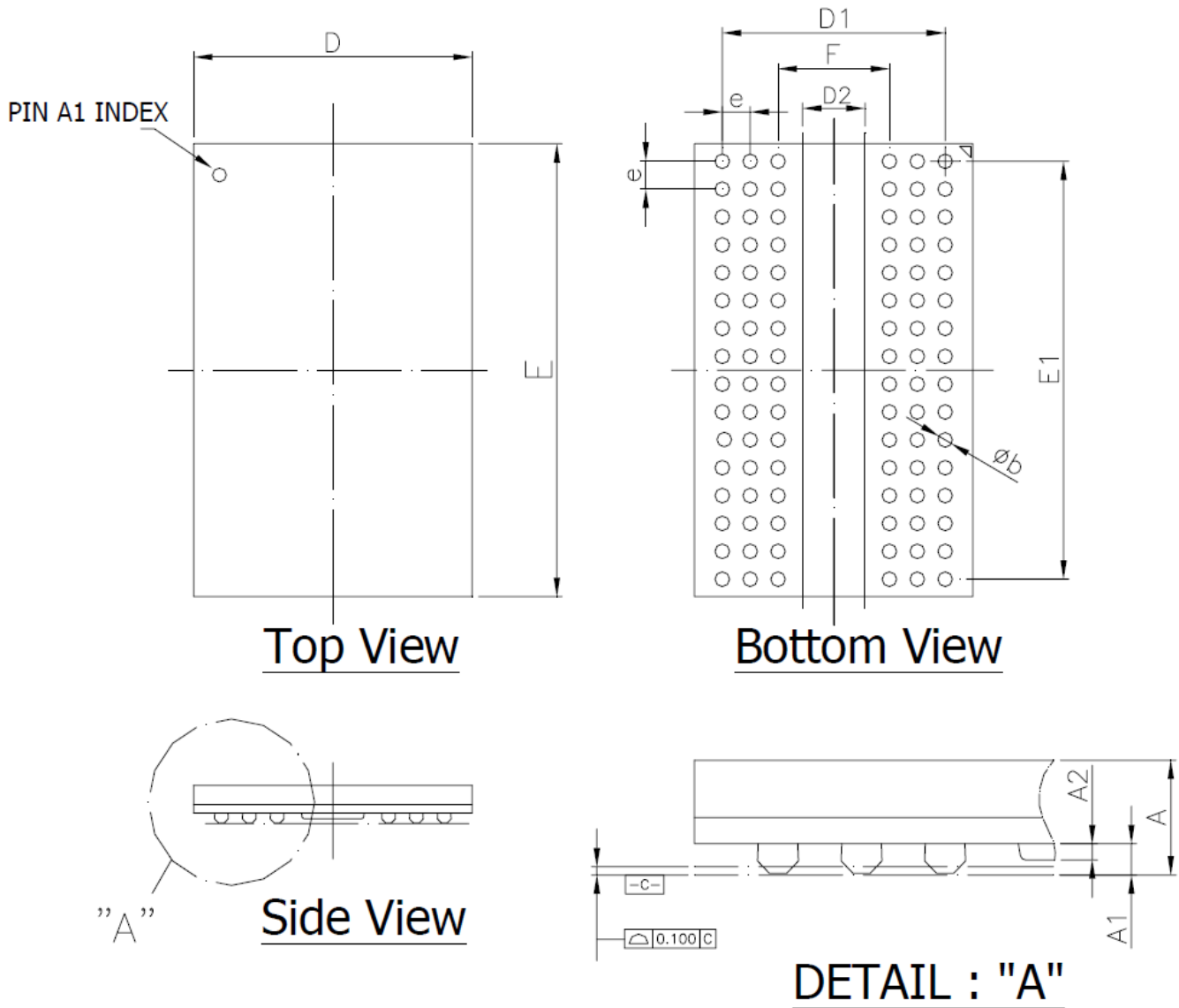
Figure 107. 96-Ball FBGA Package 8x13x1.0mm(max) Outline Drawing Information
