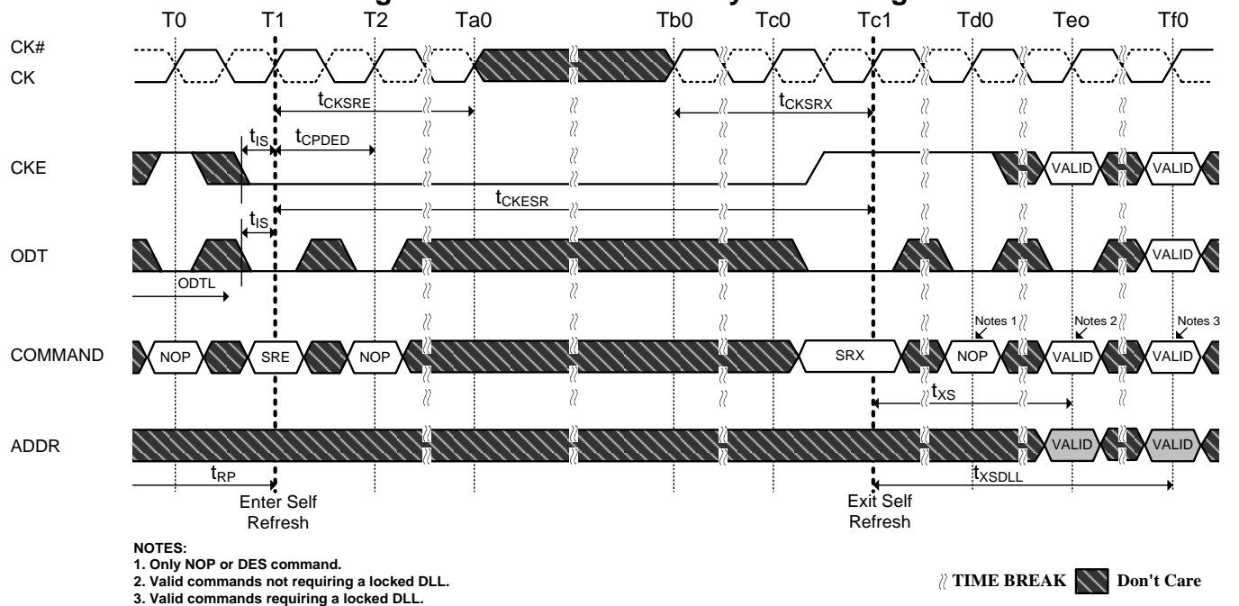
Figure 81. Self-Refresh Entry/Exit Timing
