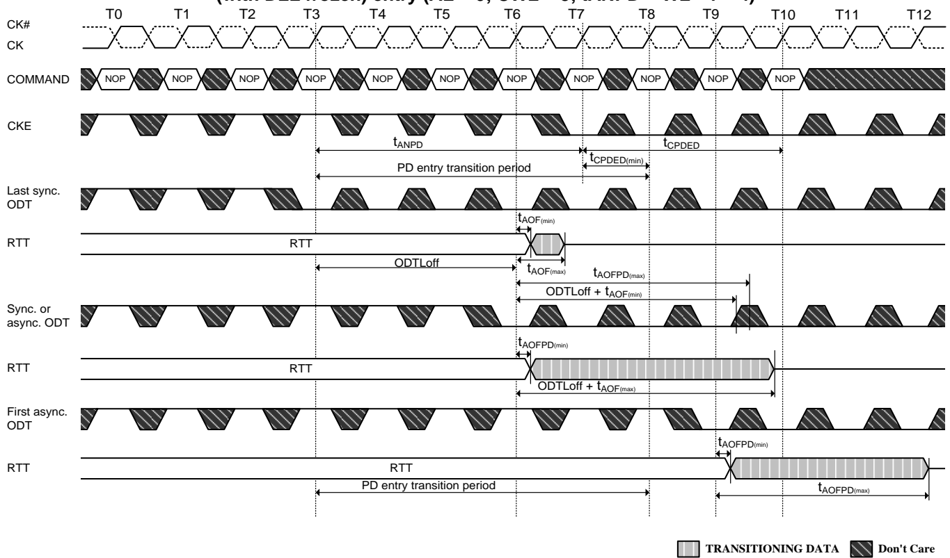
Figure 100. Synchronous to Asynchronous transition during Precharge Power Down (with DLL frozen) entry (AL = 0; CWL = 5; t_{ANPD} = WL - 1 = 4 )
