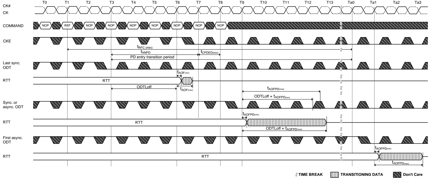
Figure 101. Synchronous to Asynchronous transition after Refresh Command (AL = 0; CWL = 5; tANPD = WL - 1 = 4)
