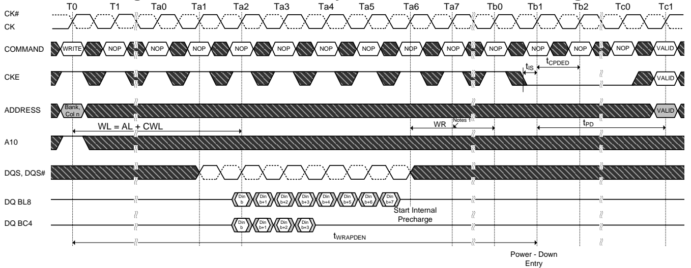
Figure 84. Power-Down Entry after Write with Auto Precharge
