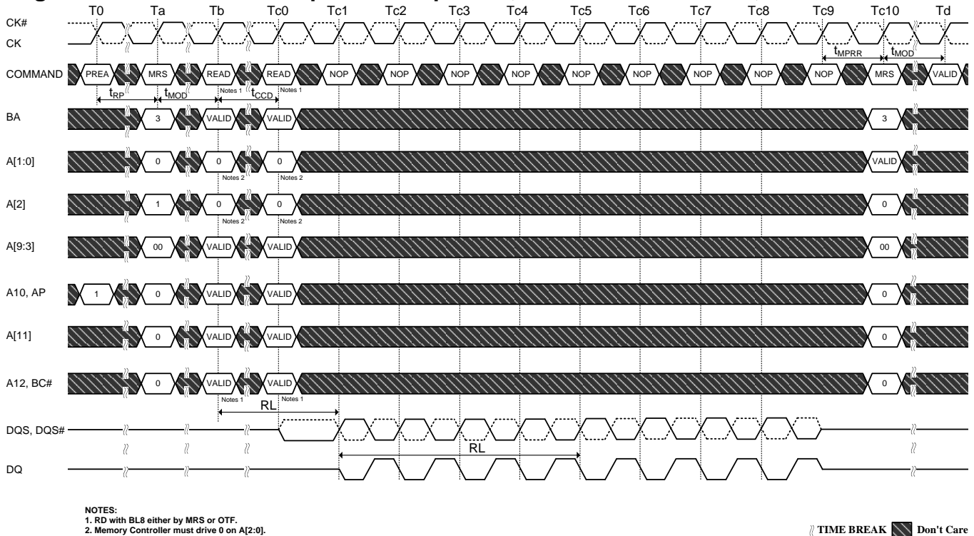
Figure 53. MPR Readout of predefined pattern, BL8 fixed burst order, back to back radout
