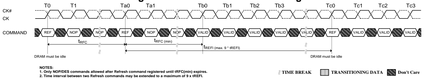
Figure 80. Refresh Command Timing
