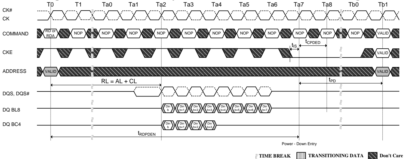
Figure 83. Power-Down Entry after Read and Read with Auto Precharge
