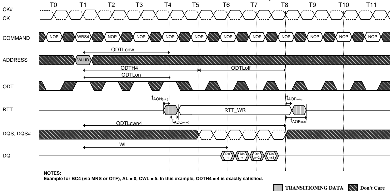
Figure 98. Dynamic ODT: Behavior with ODT pin being asserted together with Write Command for a duration of 4 clock cycles
