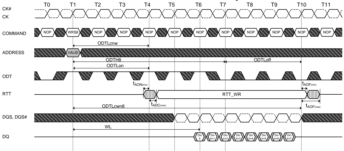
Figure 96. Dynamic ODT: Behavior with ODT pin being asserted together with Write Command for a duration of 6 clock cycles
