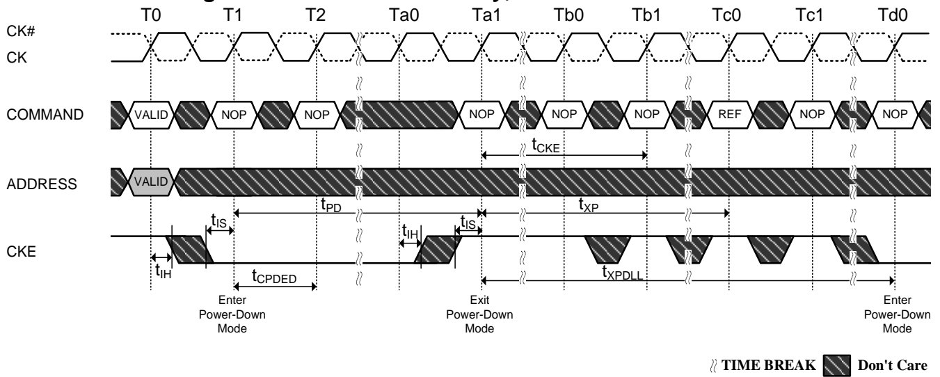
Figure 105. Power-Down Entry, Exit Clarifications-Case 2
