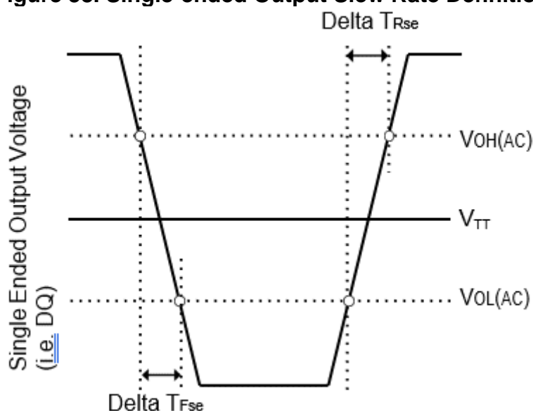
Figure 38. Single-ended Output Slew Rate Definition
