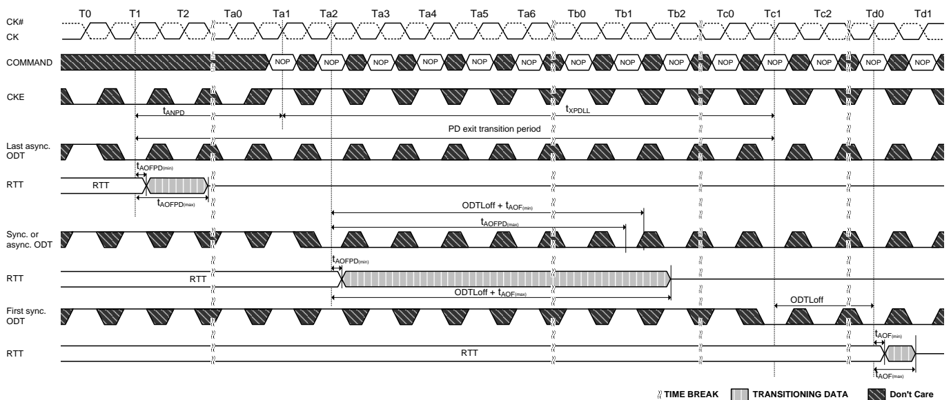
Figure 102. Asynchronous to Synchronous transition during Precharge Power Down (with DLL frozen) exit (CL = 6; AL = CL - 1; CWL = 5; tANPD = WL - 1 = 9)
