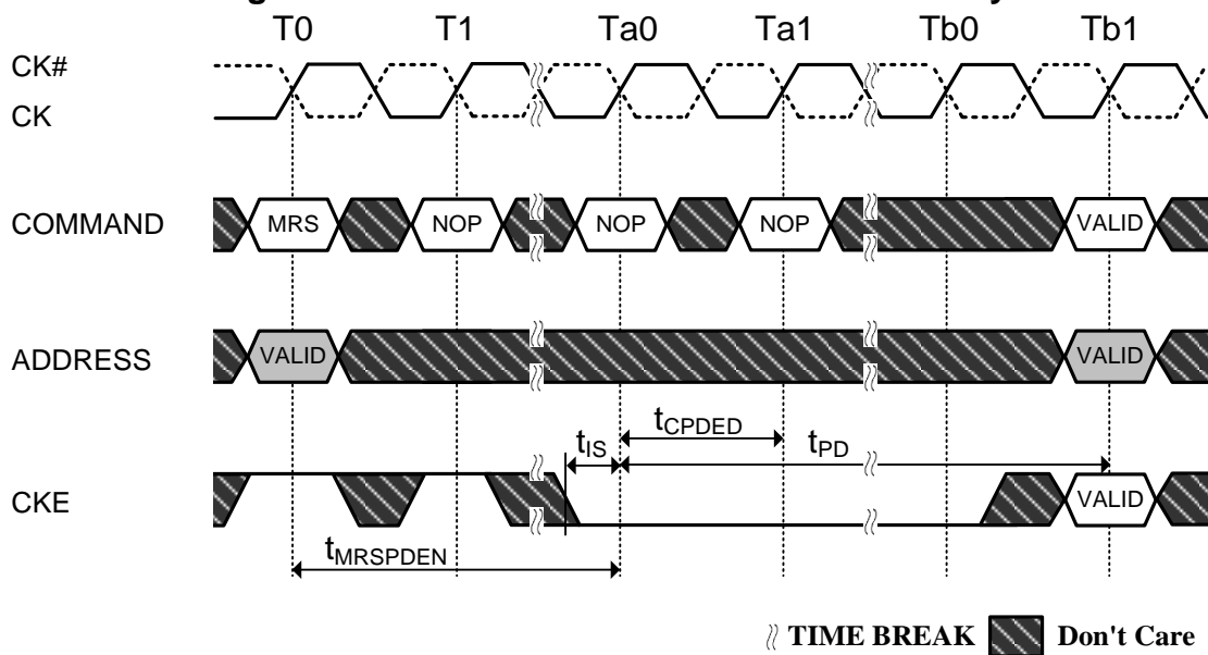
Figure 91. MRS Command to Power-Down Entry
