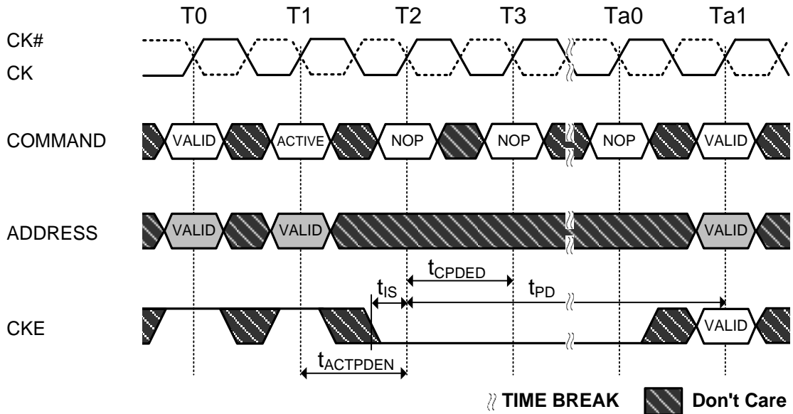
Figure 89. Active Command to Power-Down Entry
