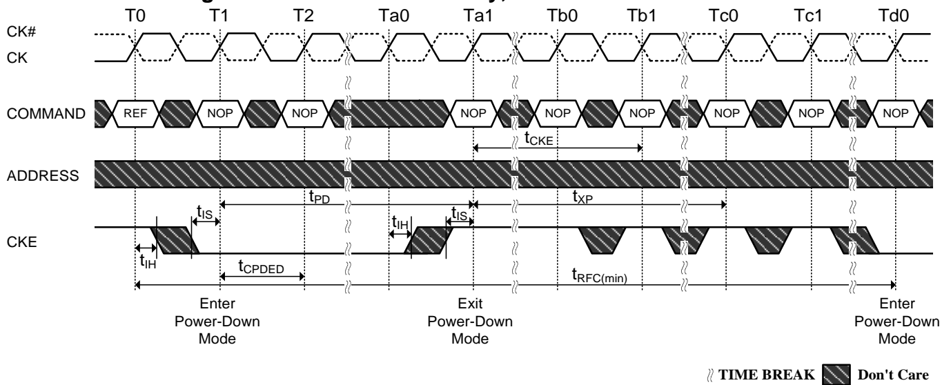
Figure 106. Power-Down Entry, Exit Clarifications-Case 3
