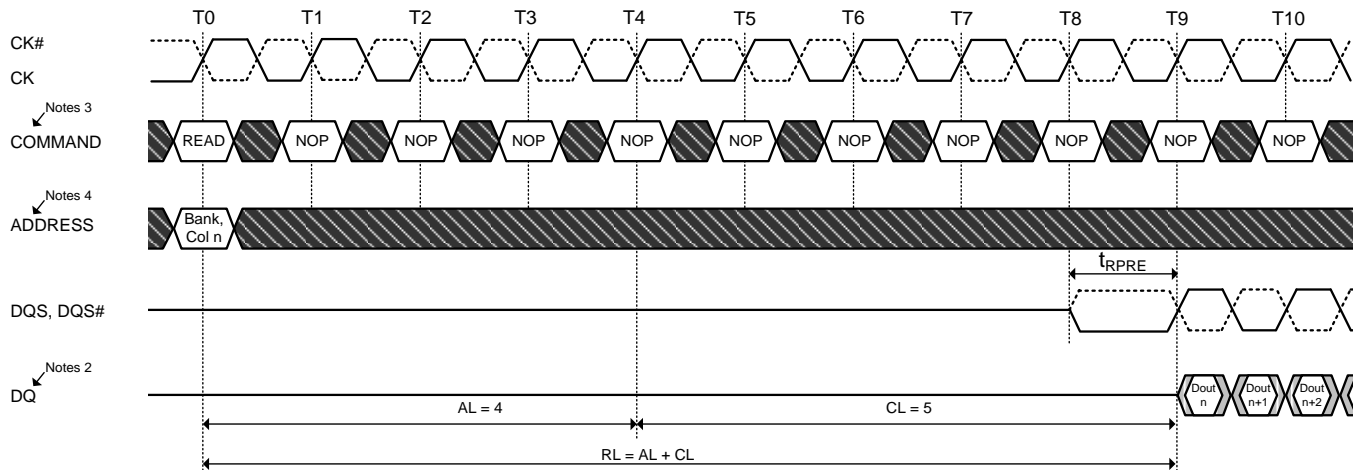
Figure 19. READ Burst Operation RL=9 (AL=4, CL=5, BL=8)
