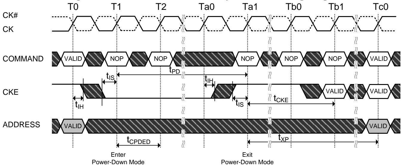
Figure 82. Active Power-Down Entry and Exit Timing Diagram
