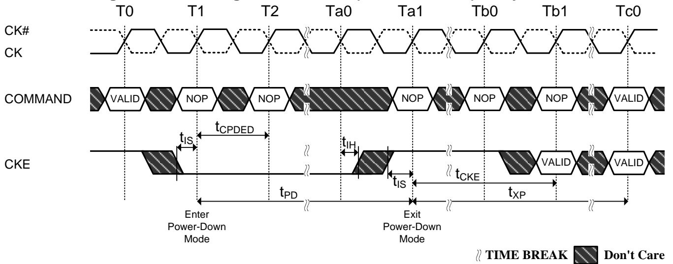
Figure 86. Precharge Power-Down (Fast Exit Mode) Entry and Exit
