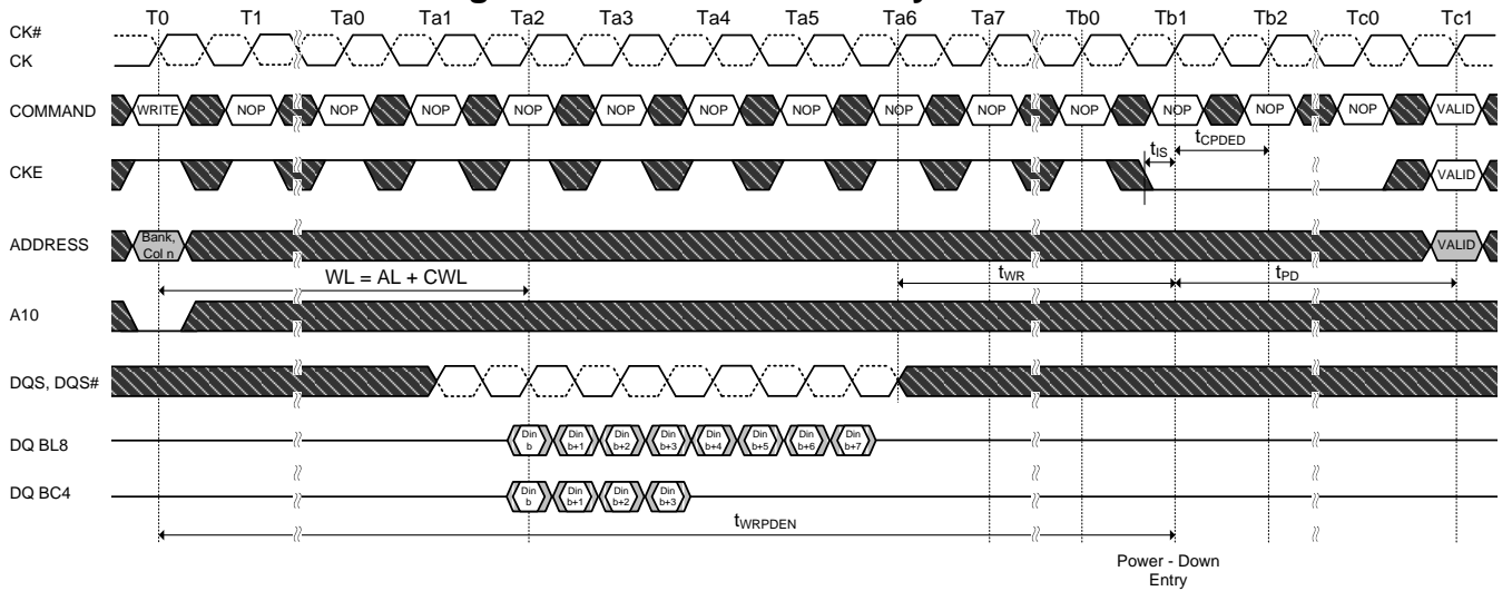
Figure 85. Power-Down Entry after Write
