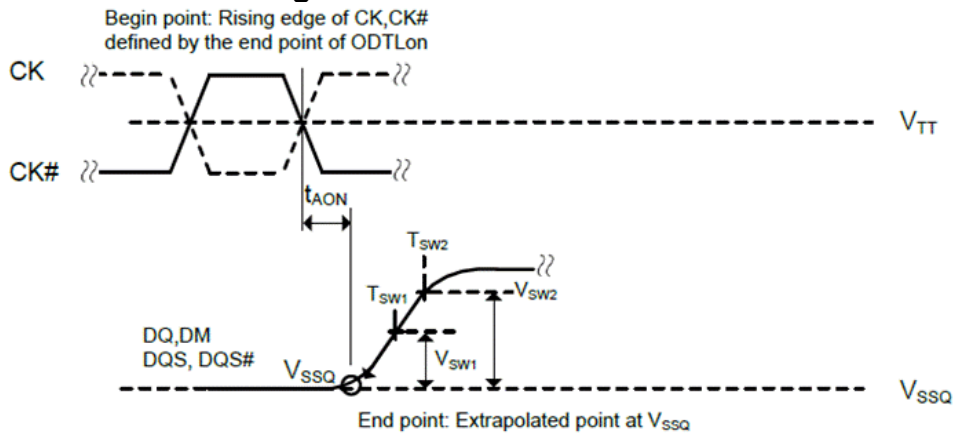
Figure 46. Definition of tAON
