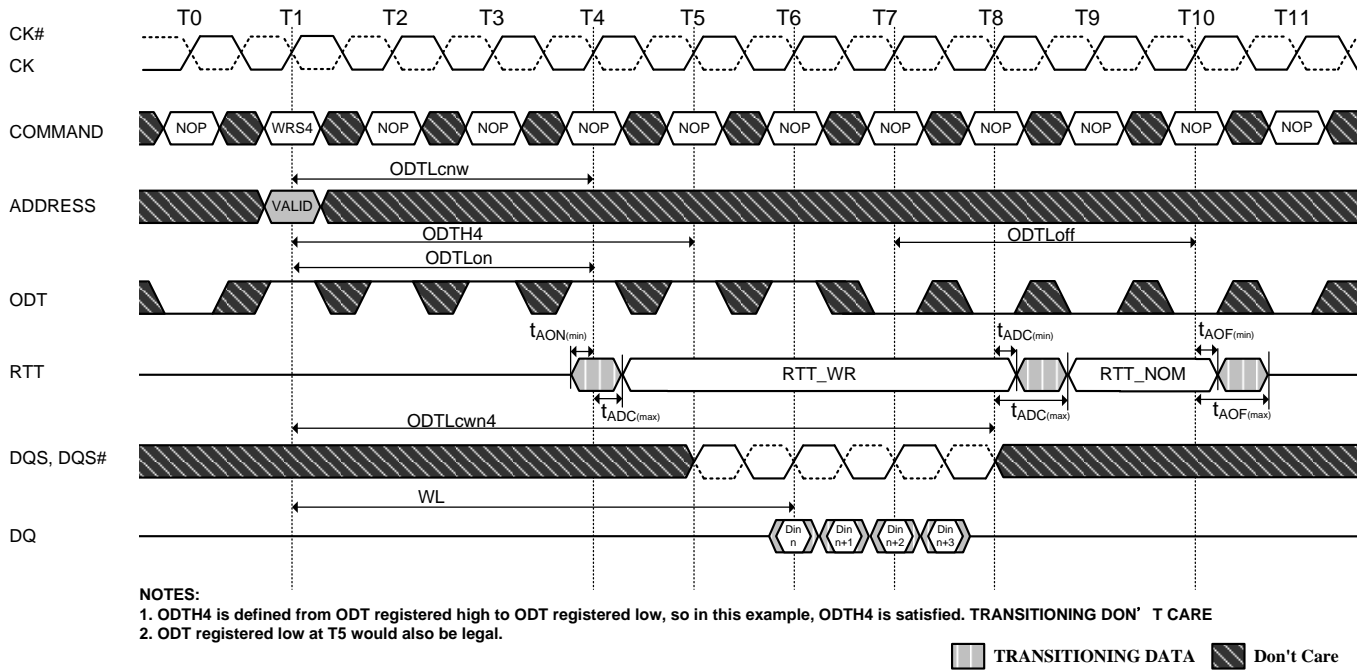
Figure 97. Dynamic ODT: Behavior with ODT pin being asserted together with Write Command for a duration of 6 clock cycles, example for BC4 (via MRS or OTF), AL = 0, CWL = 5.
