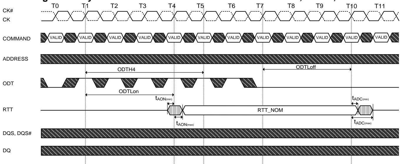
Figure 95. Dynamic ODT: Behavior without Write Command, AL = 0, CWL = 5
