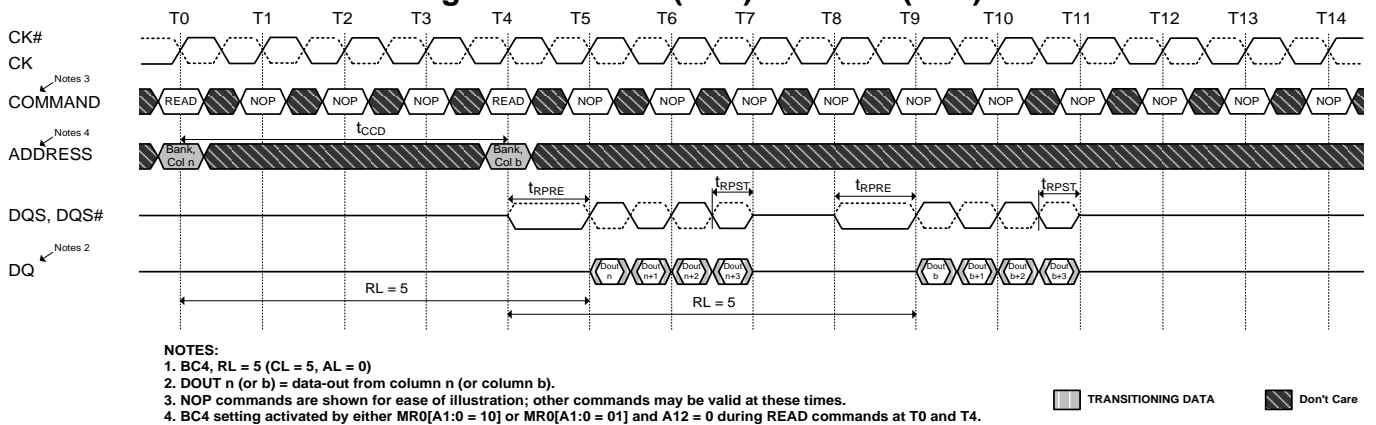
Figure 58. READ (BL4) to READ (BL4)
