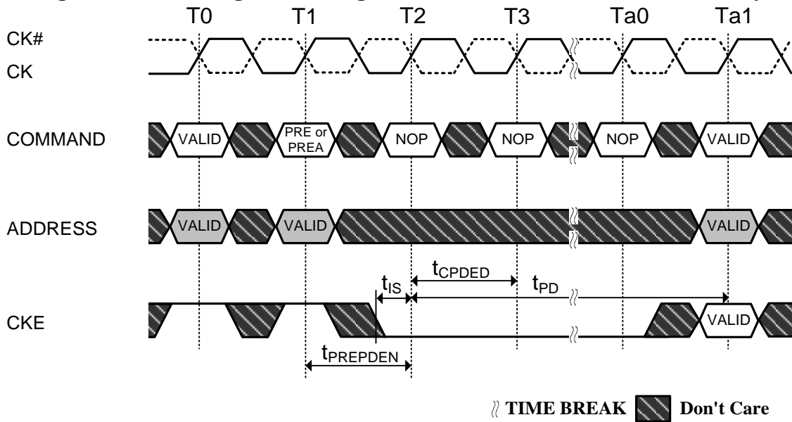
Figure 90. Precharge, Precharge All Command to Power-Down Entry
