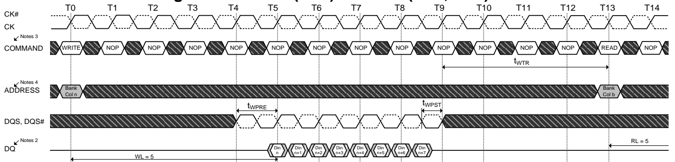
Figure 75. WRITE (BC8) to READ (BC4, BC8) OTF
