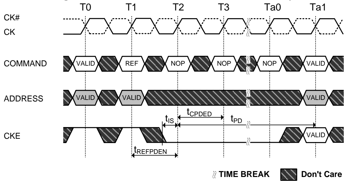
Figure 88. Refresh Command to Power-Down Entry
