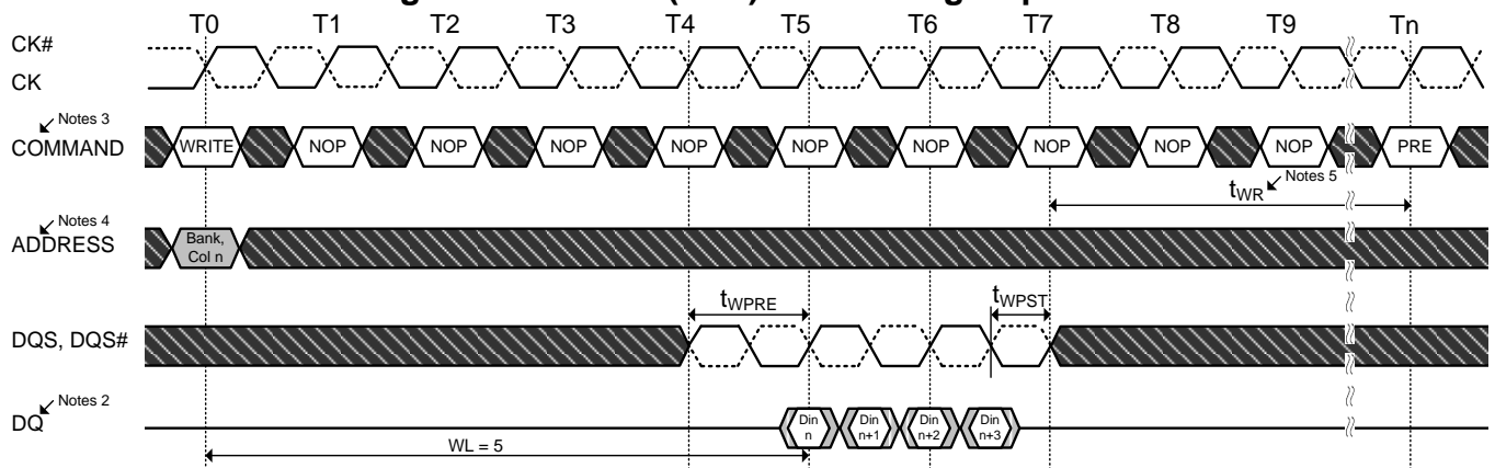
Figure 71. WRITE (BC4) to Precharge Operation
