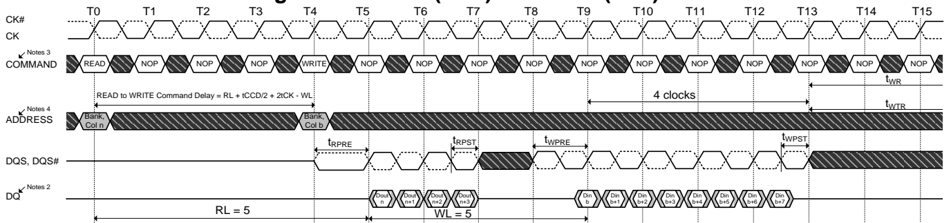
Figure 63. READ (BC4) to WRITE (BL8) OTF
