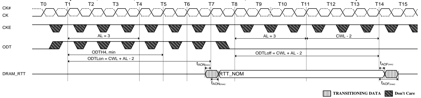
Figure 92. Synchronous ODT Timing Example
