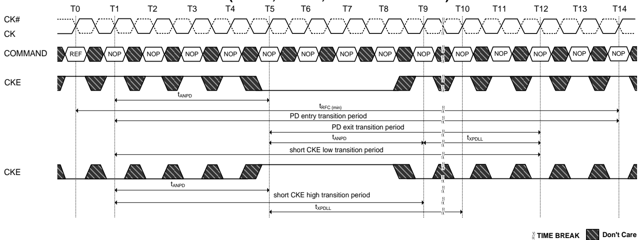
Figure 103. Transition period for short CKE cycles, entry and exit period overlapping (AL = 0, WL = 5, tANPD = WL - 1 = 4)
