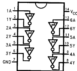
Pin Assignment for DIP, SSOP, TSSOP and SOIC
