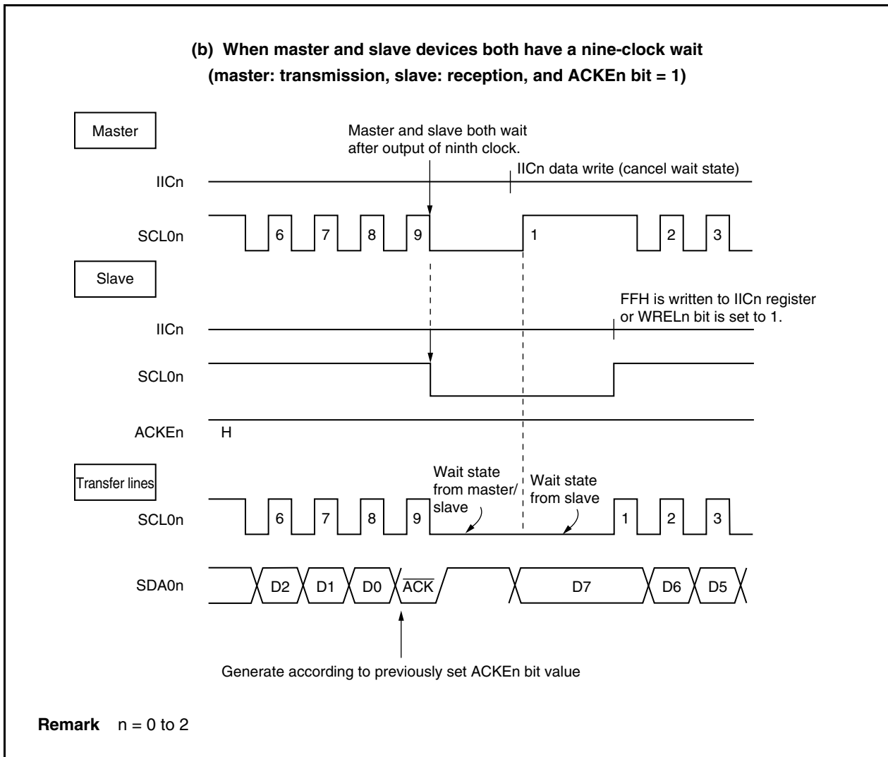
Figure 19-13. Wait State (2/2)
