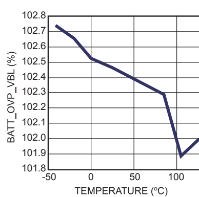
BATT_OVP_VBL_% vs. Temperature
