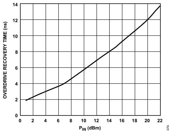
Figure 75. Overdrive Recovery Time vs. P_{IN} at 7 GHz, Recovery to Within 90% of Small Signal Gain Value, V_{DD} = 5 \text{ V} , R_{BIAS} = 4.12 \text{ k}\Omega
