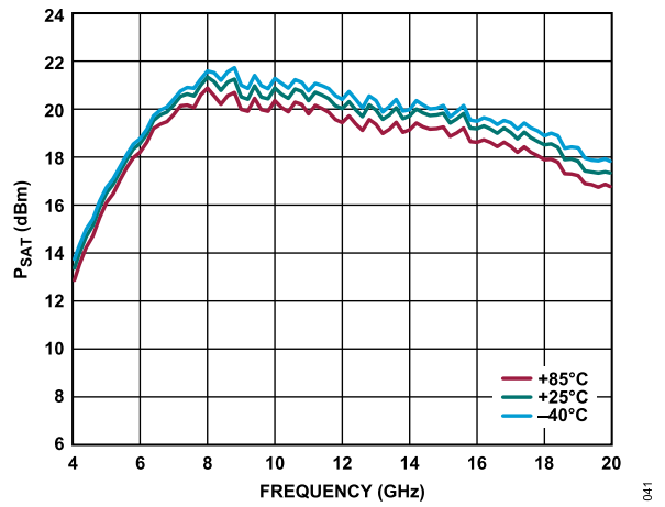
Figure 41. P_{SAT} vs. Frequency for Various Temperatures, 4 GHz to 20 GHz, V_{DD} = 5\text{ V} , I_{DQ} = 90\text{ mA} , R_{BIAS} = 4.12\text{ k}\Omega
