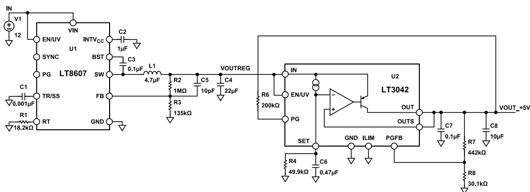
Figure 80. Recommended Power Management Circuit
