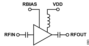
Figure 78. Simplified Schematic
