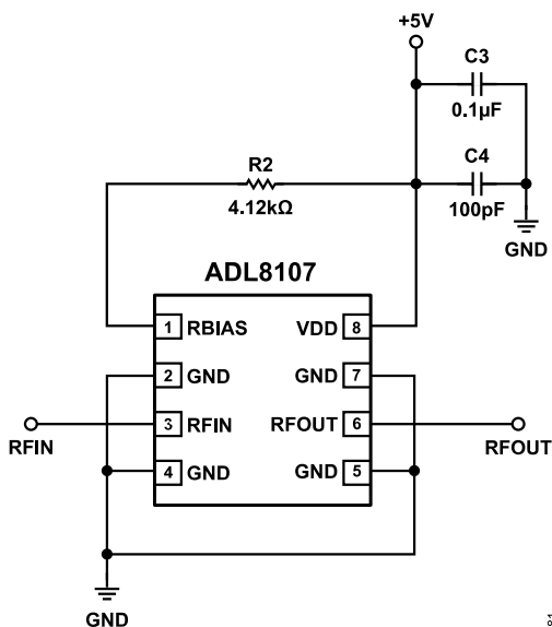
Figure 79. Typical Application Circuit
