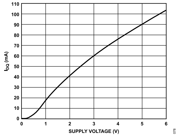
Figure 77. I_{DQ} vs. Supply Voltage, R_{BIAS} = 4.12 \text{ k}\Omega
