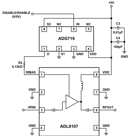
Figure 81. Fast Enable and/or Disable Circuit Using an SPDT
