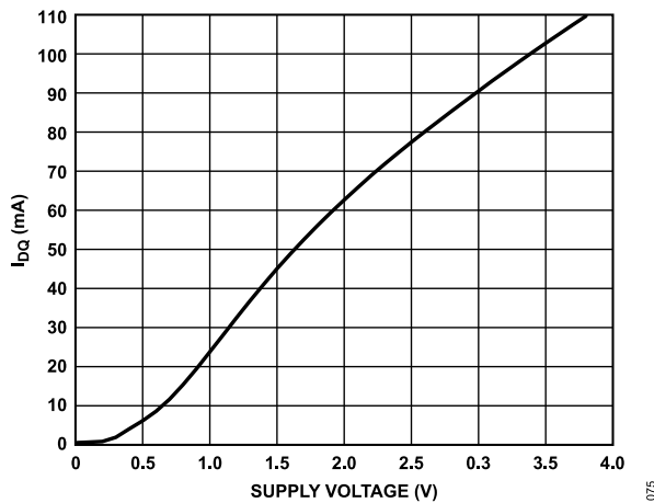
Figure 74. I_{DQ} vs. Supply Voltage, R_{BIAS} = 909 \Omega
