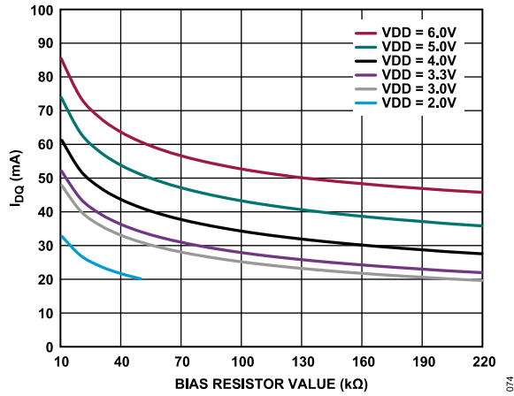
Figure 73. I_{DQ} vs. Bias Resistor Value, 10 k \Omega to 130 k \Omega , Various Supply Voltages
