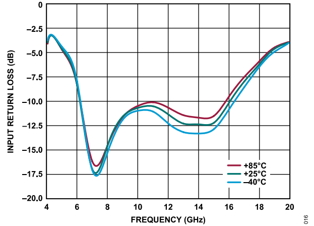
Figure 16. Input Return Loss vs. Frequency for Various Temperatures, 4 GHz to 20 GHz, VDD = 5 V, IDQ = 90 mA, RBIAS = 4.12 kΩ
