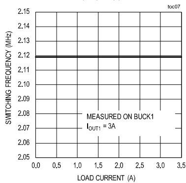
SWITCHING FREQUENCY vs. LOAD CURRENT
