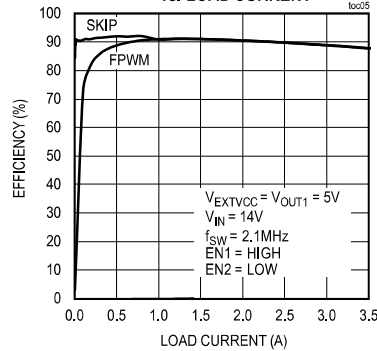
BUCK1 EFFICIENCY vs. LOAD CURRENT
