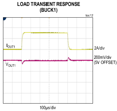
CONDITIONS: V OUT1 = 5V, f SW = 2.1MHz, FSYNC = HIGH, EN1 ONLY
