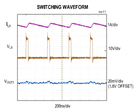
CONDITIONS: V IN = 18V, V OUT2 = 1.8V, f SW = 2.1MHz, I OUT2 = 1A
