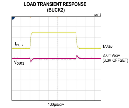
CONDITIONS: V OUT1 = 3.3V, f SW = 2.1MHz, FSYNC = HIGH, EN1 ONLY
