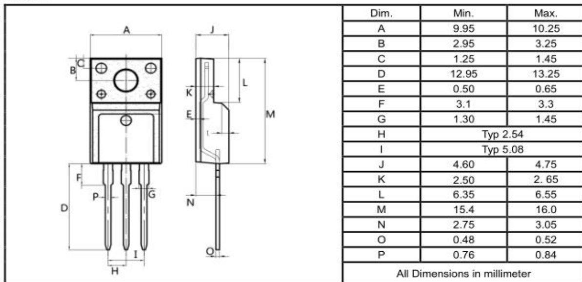
TO-220F
