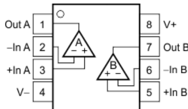
OPA2340: 8-Pin SOP-8 Top View
