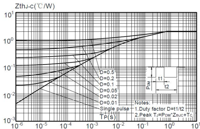
Figure.11: Maximum Effective Transient Thermal Impedance, Junction-to-Case
