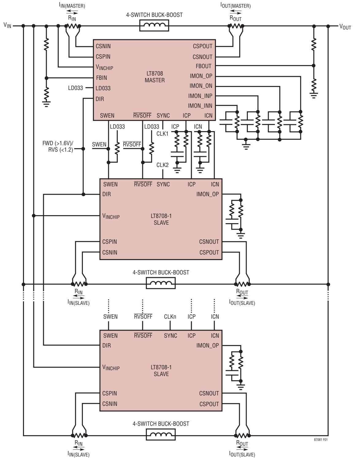
Figure 2. Simplified Multiphase Configuration Diagram
