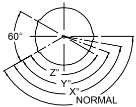
MASTER KEYWAY POSITION SIZES 7 THROUGH 15
