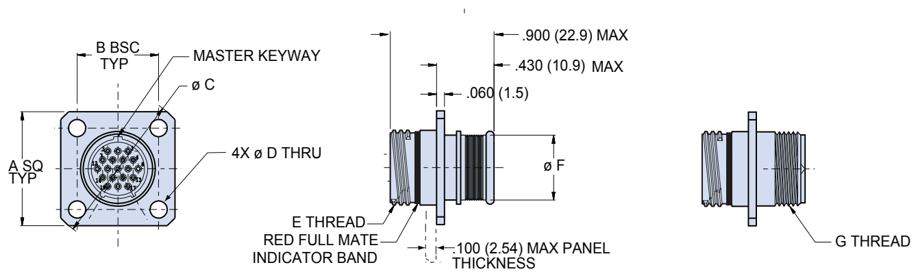
Integral Band Platform 801-009-02
