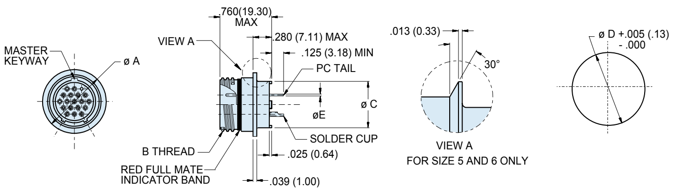
Solder Mount Hermetic 801-012-03
