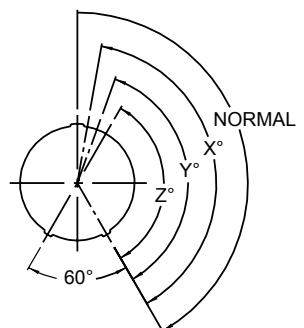
MASTER KEYWAY POSITION SIZES 5 THROUGH 6
