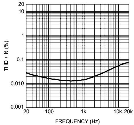
THD+N vs Frequency V_{DDLS} = 5V , V_{DDHP} = 2.75V , R_L = 32\Omega SE, P_O = 20mW/Ch , Mode 8 (Left/Right), 80kHz BW
